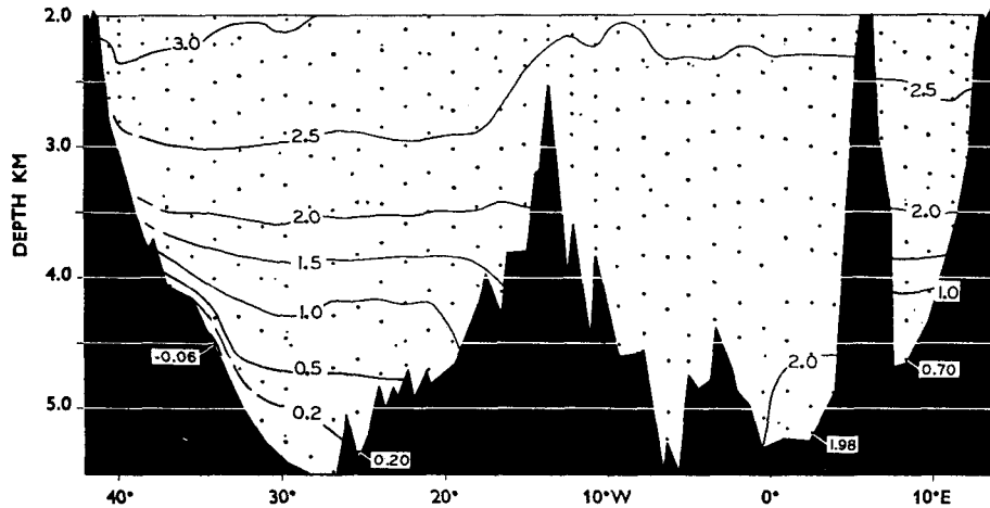
Figure 1. Potential temperature ( ^{\circ}\text{C} ) at depths greater than 2000 m in a section along 24^{\circ}\text{S} in the Atlantic Ocean. The contour interval is 0.5^{\circ}\text{C} except for the dashed line. The major topographic features are South America on the left, the Mid-Atlantic ridge, the Walvis Ridge, and Africa on the right.
