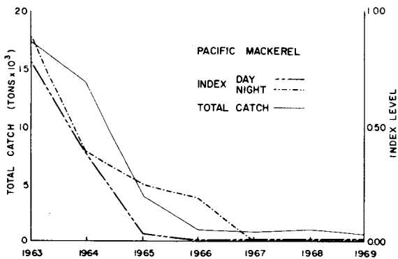
FIGURE 5.—Total catch, average index values for the Pacific mackerel.
