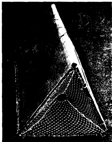
Figure 5.—A collapsible tent trap ready for fishing.
