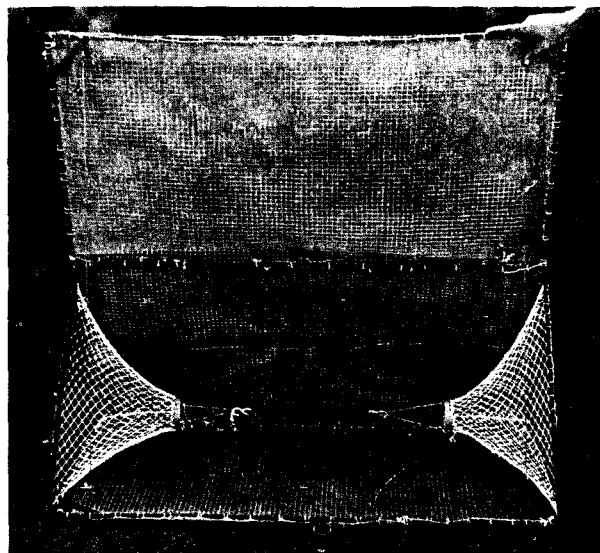
Figure 6.—A tent trap with raised lid.
