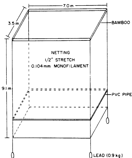
FIGURE 5.—Diagram of an acoustically transparent trap for ensnifing a group of fish of known size and weight.
