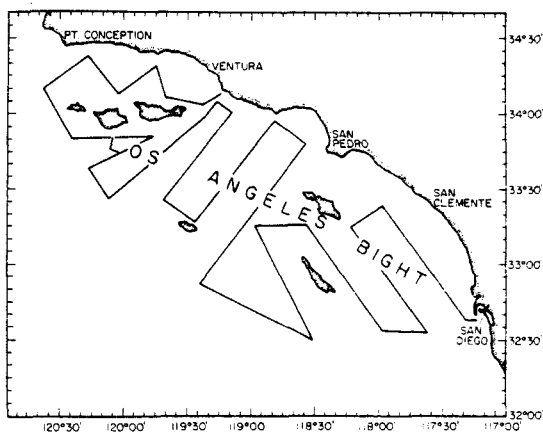
FIGURE 8.—Los Angeles Bight including a 721-mile sonar survey track transected twice, 17-26 September 1974.
