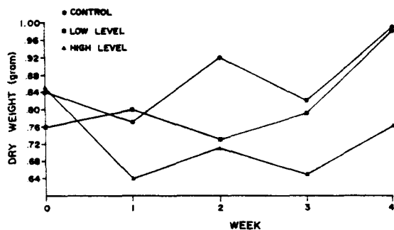
FIGURE 1.—Average weight of each of three groups of striped bass, Morone saxatilis , exposed to three concentrations of benzene (0, 3.5, and 6.0 \mu\text{l/liter} ) for 4 wk. The dry weight of high-level exposure fish was significantly less ( P < 0.01 ) than the other two groups at the end of the first week and thereafter. The dry weight of the three groups combined was significantly higher ( P < 0.05 ) than in previous weeks.
