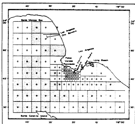
FIGURE 7.—Stations at which the ratio of o,p' DDE to p,p' DDE was greater than 0.40:1.00.
