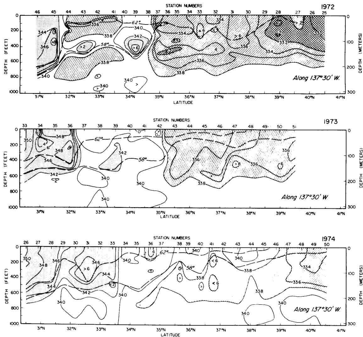
FIGURE 8.—Vertical sections of temperature and salinity along long. 137°30' W during June 1972, 1973, and 1974. Low salinity water (<33.8‰) indicative of Subarctic water is hatched and crosshatched. High salinity water (>34.2‰) indicative of Central water is shaded with a dot pattern. The 58° and 62 F isotherms are shown by heavy dashed lines.
