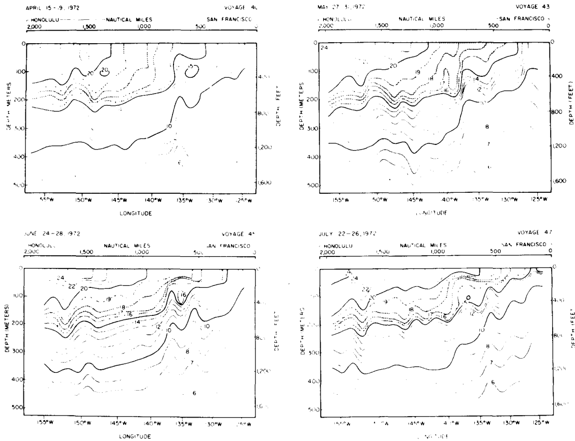
FIGURE 14.— Vertical temperature sections on a transect from Honolulu to San Francisco during April to July 1972. The temperature range between 16° and 19° C (60.8° and 66.2° F) is shaded.
