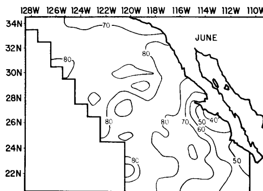
FIGURE 15. Cloud cover during June. Means of reported cloud amounts were computed by 1 degree squares during the month of June. Units are percent of sky obscured.
