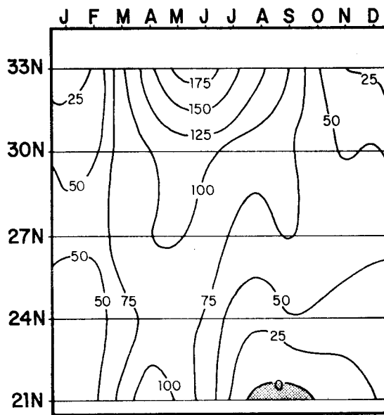
FIGURE 21. Mean values by month and position of 6 hourly coastal upwelling indices for the 7 year period, 1967-73. Locations are indicated by large dots in Figure 1. Units are m^3 per second per 100 m of coast. Negative values are shaded.
