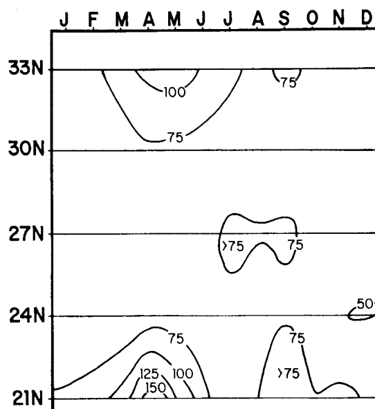
FIGURE 22. Standard deviations of monthly distributions of 6 hourly coastal upwelling indices. Locations are indicated by large dots in Figure 1. Units are m^2 per second per 100 m of coast. Period covered is 1967-73.
