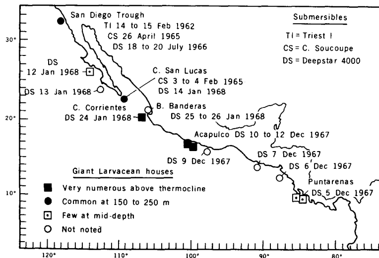
Fig. 1. Locations and dates of submersible dives and the observed relative abundance of large larvacean houses.
