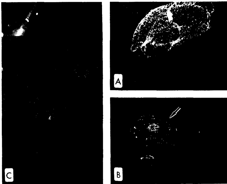
Fig. 2. Photographs of large larvacean houses taken during deep submersible dives. (A) Type 1 house, about 70 to 100 cm in its greatest dimension, at a depth of 200 m in the San Diego trough, 26 April 1965. (B) Type 2 houses, about 20 to 26 cm in length, at a depth of 120 m off Cabo San Lucas, Baja California, 4 February 1965. The arrow marks the probable intake filter. The organism below the house is a pelagic gastropod, probably Pterotrachea coronata . (C) The type 3 house at a depth of 40 m off Cape Corrientes, Mexico, 24 January 1968. The houses are about 30 to 40 cm in diameter and were disintegrating in the vortex caused by the submersible's movements. The bottom of the intake funnel of the collecting device (upper left) is 27 cm across. In all the houses the internal filters show clearly. The larvaceans, if present, should be closely associated with these structures although they cannot be made out in the pictures.
