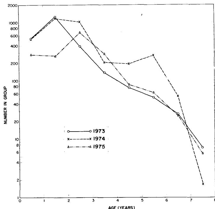
Figure 12.— Catch curve for bigeye tuna.
