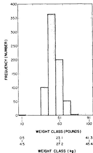
Figure 8.—Frequency distribution of weights of albacore caught in the night handline fishery for tunas.
