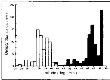
Figure 2.—Pacific ocean perch density (dark bar) and chilipepper density (clear bar) in pounds per nautical mile.
