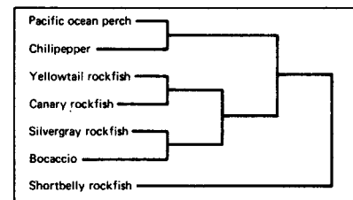
Figure 1.—Cluster analysis of morphological similarity of rockfish species.
