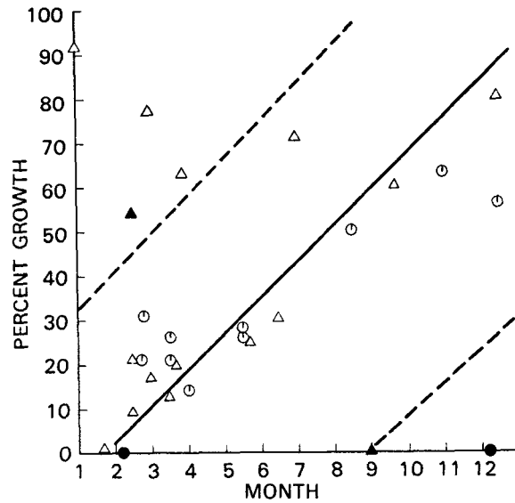
Fig. 4. Scatterplot of the percent growth of the last GLG in teeth of young Tursiops on approximate date of death. Percent growth calculated for each animal from actual width of the last layer divided by the average total width of the GLG. Solid line presents expected growth of the GLG throughout the year if the GLG begins in late Jan.-early Feb. and grows at a constant rate. Hatched line represents the same for GLGs which begin in September. Circles are females, triangles are males. Hollow symbols indicate an opaque last layer, solid symbols represent a translucent last layer.
