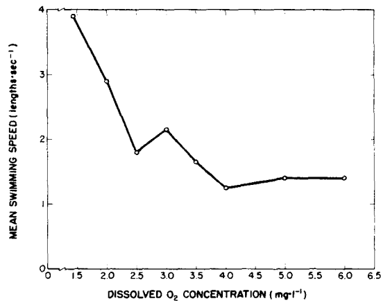
FIGURE 7.—Relation between mean swimming speed and dissolved oxygen concentration. The data for O_2 of 6.0 and 5.0 mg \cdot l^{-1} are from the oxygen-uptake experiments. Those at lower concentrations are derived from the low-oxygen tolerance experiments. Length measure is fork length.
