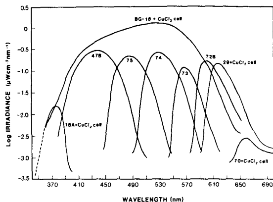
Figure 2. The spectral irradiance of the color filters used in the experiment. Filters used are given at top of each curve. All are Kodak with the exception of the Schott BG-18. BG-18 + \text{CuCl}_2 is the filter used for the broadband blue-green light treatments. The other filters are color filters, with maxima (from left to right) of 370 nm, 440 nm, 485 nm, 530 nm, 570 nm, 600 nm, 620 nm, and 660 nm. The irradiance below 362 nm in 18A is estimated from the curve drawn by eye (dashed).
