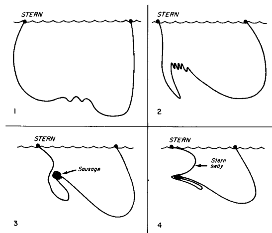
Figure 14.—Backdown channel cross section showing development of stern sway during backdown.
