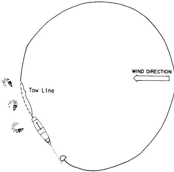
Figure 9.—Always set after turning into the wind. This will keep the net upwind of the vessel.
