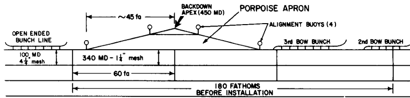
Figure 16.—Configuration of porpoise safety panel and super apron.
