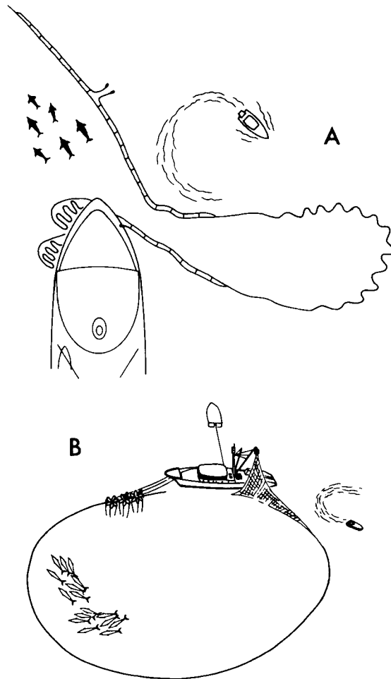
Figure 11.—Use speedboats to prevent porpoise from (A) entering dangerous areas of the net and (B) from entering the area where the corks come out of the water during net roll. Corks make good sonar targets for the porpoise while 106 mm (4¼-in) mesh may not.
