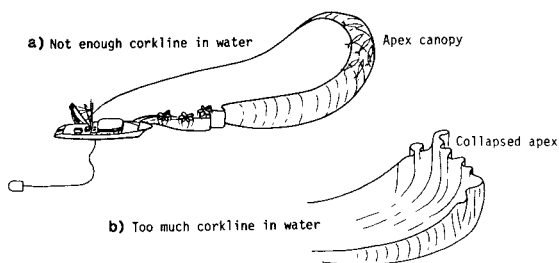
Figure 13.—To ensure the proper amount of corkline for backdown, clearly mark tie-down points for the net and last bow bunch pulled. Never estimate these points. The proper amount of corkline is directly related to the depth of the net. Too little corkline (a) in the water will result in apex canopies. Too much corkline (b) will produce a collapsed and wrinkled corkline.
