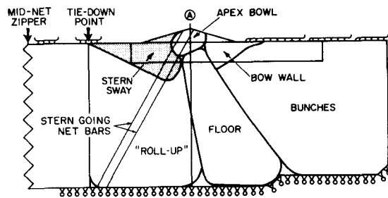
Figure 12.—Functional distribution of webbing in a stabilized backdown channel.
