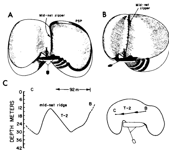
Figure 8.—A. Mid-net zipper ridge when fully pursed. Note indentation of cork-line opposite vessel. B. Zipper ridge with one-fourth net retrieved aboard vessel. C. Fathometer trace when fully pursed.
