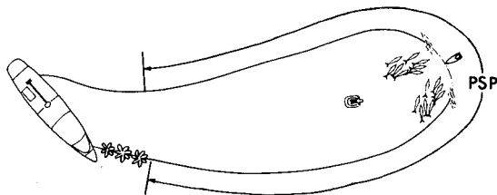
Figure 17.—Porpoise safety panel (PSP) must cover the perimeter of the backdown channel, at least from the last bow bunch pulled, around the apex and sternward at least two-thirds of the distance back along the sternside of the channel.
