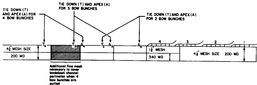
Figure 18.—Multiple tie-down points for backdown in nets without aprons when using 2, 3, or 4 bow bunches. Remember to avoid placing bunchlines within 18 m (10 fathoms) of any of the apex markers.
