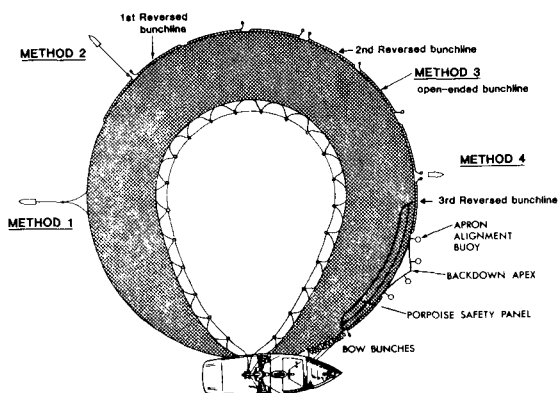
Figure 3.—Purse seine towing points for holding net open using speedboats. The three reversed bunchlines should be strategically located around the perimeter of the net but should not interfere with the porpoise apron (Method 4). Speedboats may at times find it better to pull only one regular bunchline from its end (Method 2), or from its center if its open-ended (Method 3). Speedboats may also pull directly on the corkline (Method 1) to remove small net collapses and canopies.
