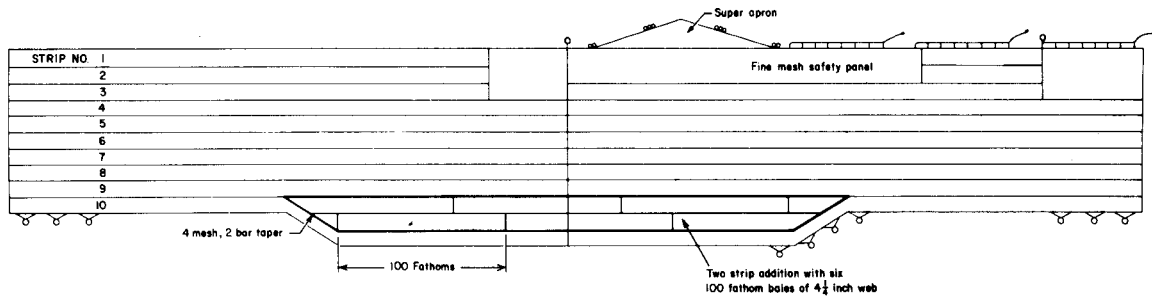
Figure 7.—A two-strip addition in the center of a 10- or 12-strip net can be accomplished with 5, 8, or 10 bales of web, depending on the length of net. The addition is installed between the last strip and the strip above. When only six 100-fathom bales are used, the top edge of the addition will measure 360 fathoms while the shorter bottom edge measures 240 fathoms. Note: New tie-down points must be determined for backdown anytime the depth of the net is changed.
