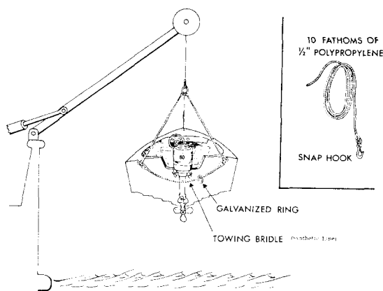
Figure 5.—Rigging for speedboat towing bridle. Note that the galvanized ring is free to slide the entire length of the towing bridle.
