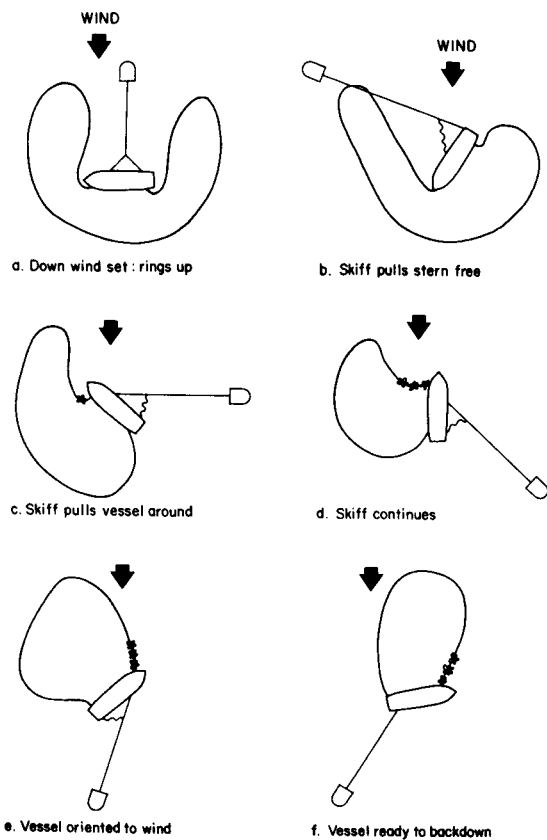
Figure 10.—Procedure for turning vessel around after making a downwind set.
