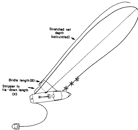
Figure 15.—Determining proper tie-down points for backdown: The sum of the calculated stretched depth (in fathoms), the length of one ring bridle, and the distance from the ring stripper to the point on the vessel where the net is tied down, gives the tie-down point within 4 or 7 m (2 or 3 fathoms).
