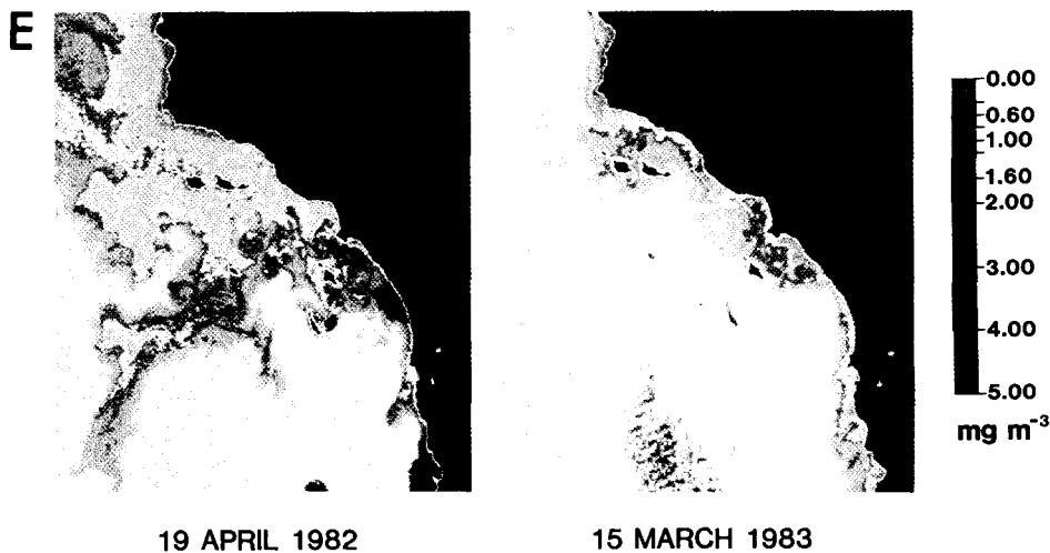
Fig. 1. Advanced Very High Resolution Radiometer sea-surface temperature images off southern California (B), central-northern California (C), and Oregon-Washington (D); Coastal Zone Color Scanner phytoplankton pigment images off southern California (E).
