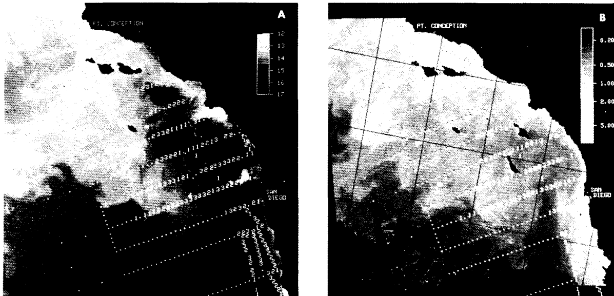
Figure 3. — Northern anchovy egg distribution, 20 March-10 April 1980; • = 0, 1 = 1-4, 2 = 5-17, 3 = 18-245 eggs/0.05 m 2 . Top photo (A) is sea surface temperature (°C) from NOAA-6 AVHRR, 7 April 1980; Photo B is of phytoplankton pigments (mg m -3 ) from Nimbus-7 CZCS, 8 April 1980.
