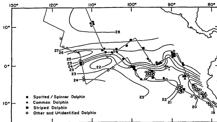
FIGURE 9.—Distribution of dolphin schools in the equatorial region during October-November 1977, relative to surface isotherms ( ^{\circ}\text{C} ). Notice the Equatorial Front or zone of rapid temperature change just north of the Equator. Clumping of sightings along the track is due to nighttime travel by ship. "Other" dolphins are primarily pilot whales.
