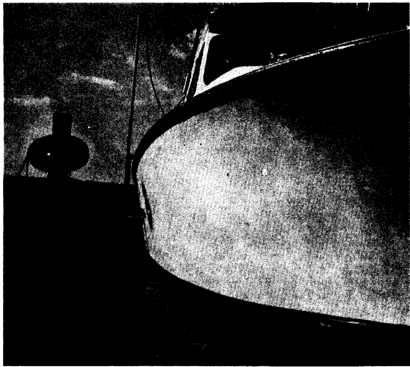
Figure 2.—Hydrophone Mounting. Top: The tracking hydrophone is in retracted position. Two triangular aluminum brackets mounted above the waterline allow the hydrophone to be lifted out of the water when not in use. Bottom: The hydrophone mounting pole is lowered through the support brackets to a position in which the hydrophone is clear of the keel and is unaffected by turbulence from the boat hull.
