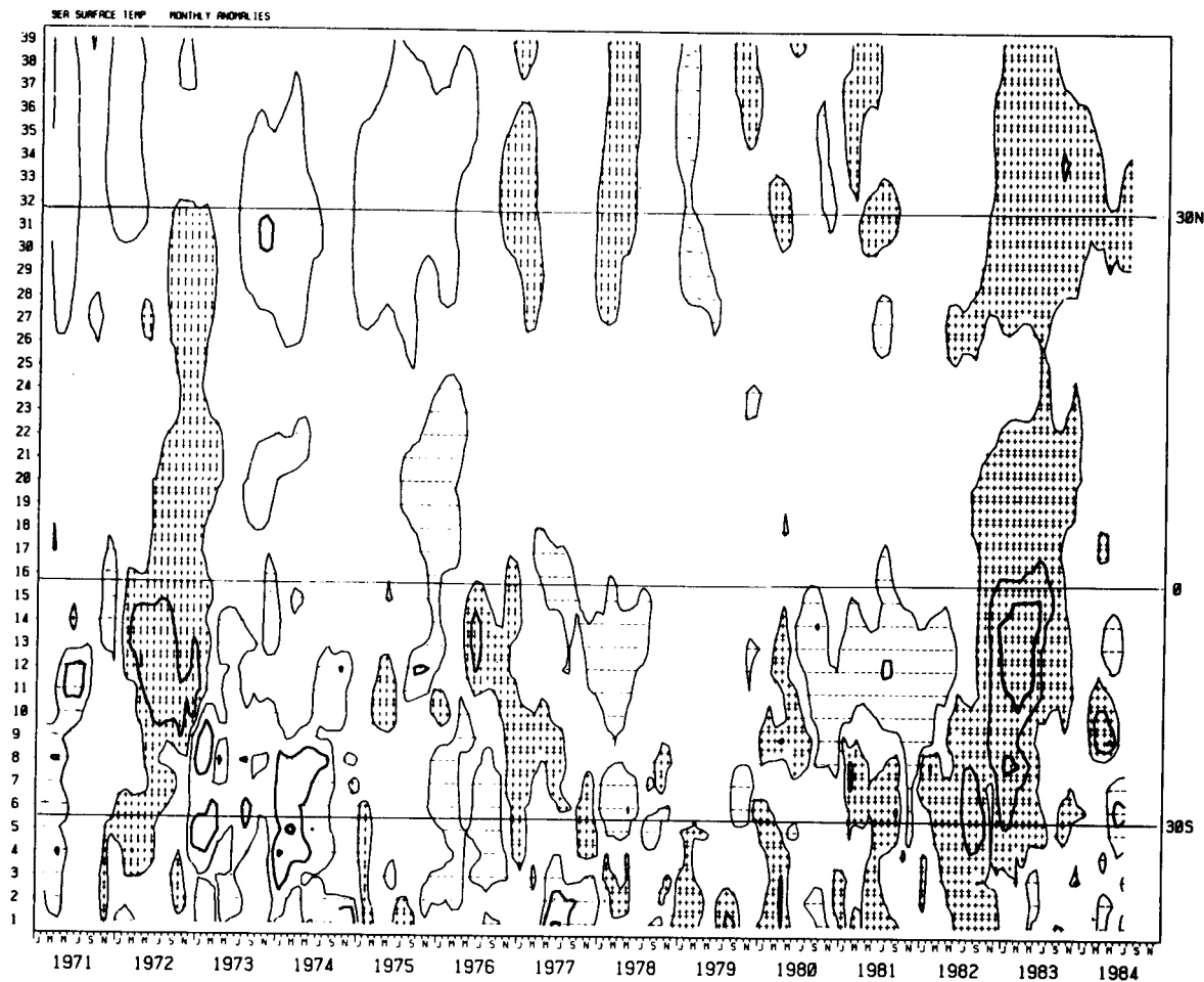
Figure 3. Anomaly of monthly mean SST along eastern boundary of Pacific Ocean. Small plus and minus signs represent anomalies before smoothing of greater than +0.5°C and less than -0.5°C, respectively. Contouring was performed after median and linear filtering. Light contour lines represent +0.5° and -0.5°C; dark contour lines represent -2.5°, -1.5°, +1.5°, and +2.5°C.
