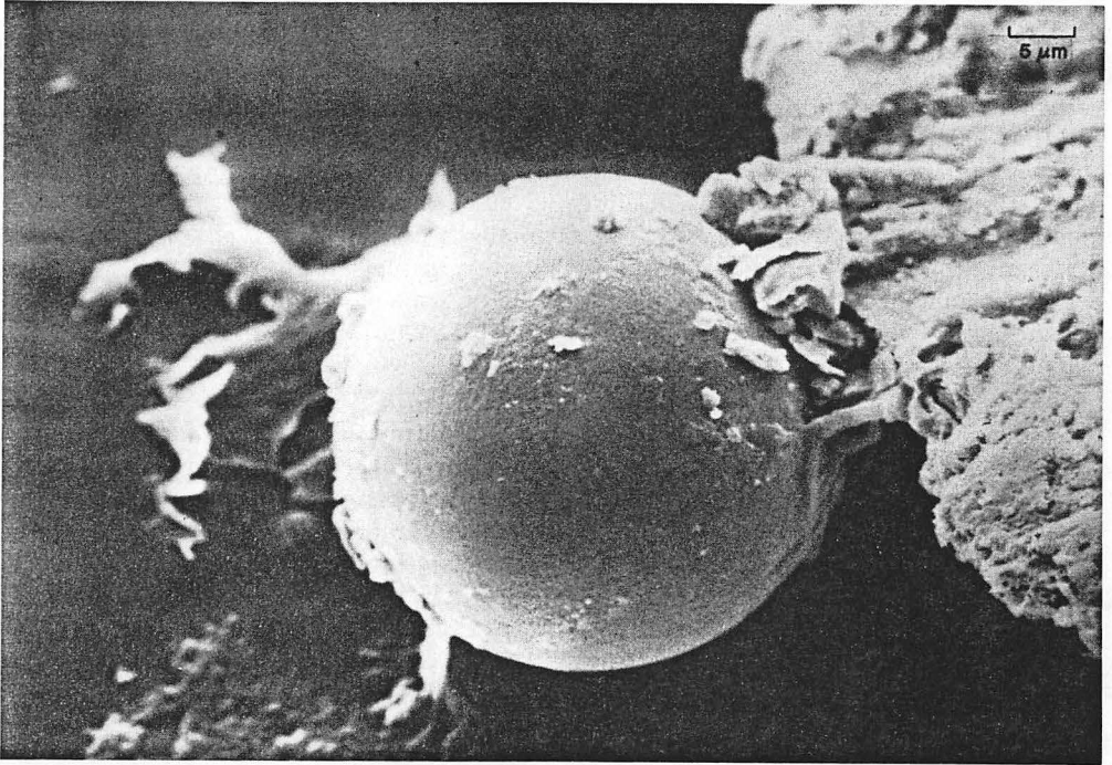
Figure 6. Scanning electron micrograph of sphere from green turtle dura mater sample.
