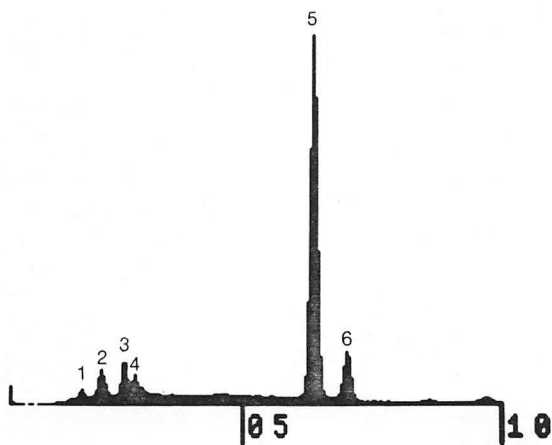
Figure 4. EDAX spectrum for magnetite sample from green turtle dura maters. Numbered peaks correspond to the following elements: 1, silica (from glass coverslip sample was placed on); 2, gold (from gold/palladium coating sprayed on sample to increase conductivity for scanning electron microscopy); 3, chlorine (from bleach used to digest dura membrane tissue); 4, palladium (from gold/palladium coating); 5 and 6, iron.
