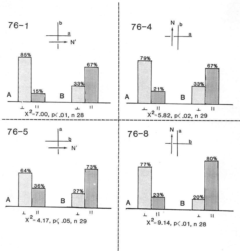
Figure 1. Results of tests with salamander groups A and B, previously trained in corridors a and b, respectively. These tests represent the four possible combinations (insets) of the expected magnetic directions relative to the home corridors and the topographical axis. The histograms show the percentage of each group of animals which moved perpendicular and parallel to the natural or altered field. For example, in test 76-1, animals in group A, which were originally trained to move perpendicularly to the magnetic field, do so preferentially (85%) even though the corridor perpendicular to the magnetic axis (b) is not their home corridor; this preferred movement also coincides with the topographical axis (represented by the vertical axis in each inset). For statistical purposes, the combined number of A- and B-group animals which moved along the expected axis is tested (chi-square, one-tailed, one degree of freedom) against the null hypothesis of a 50:50 distribution of both groups along the two perpendicular axes. From Phillips (1977).
