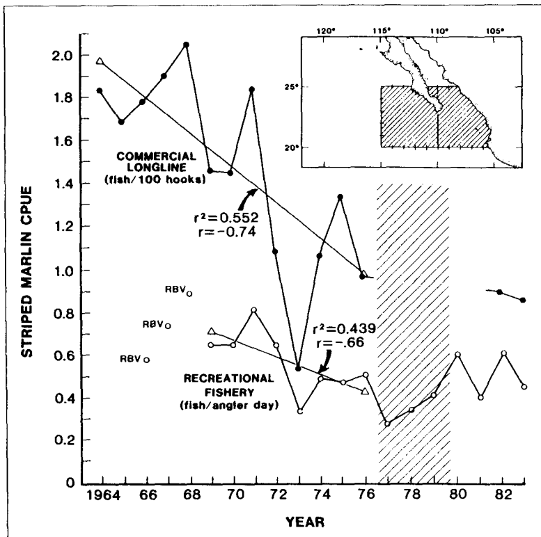
Figure 7.—Striped marlin CPUE and its regression for the commercial longline fleet 1964-76, two 5° long. by 5° lat. areas, and the Billfish Angler Survey for the southern portion of Baja California. The hatched area represents a period when longline operations were negligible within Mexico's 200-mile economic zone.
