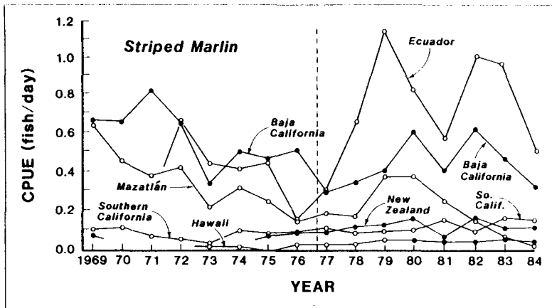
Figure 3.—Catch rates for striped marlin in areas having greater than 2,000 angler days.
