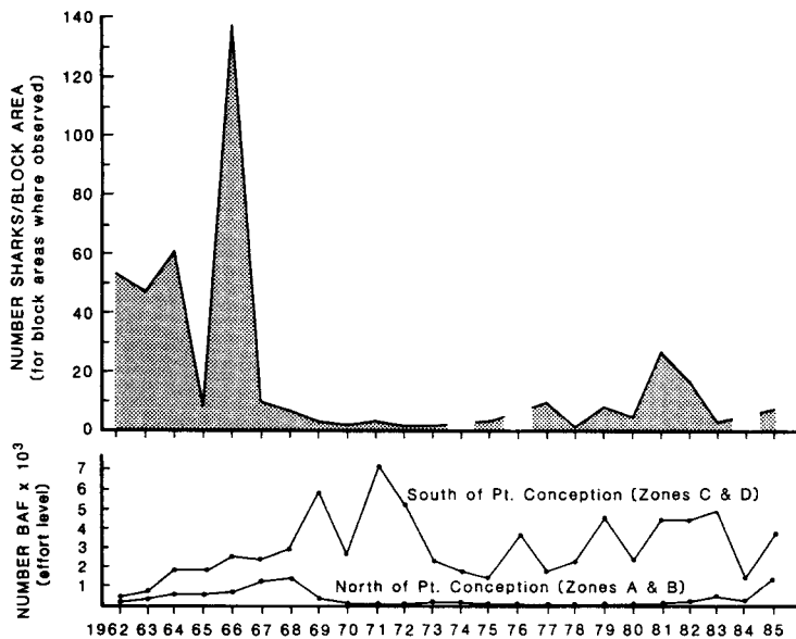
Figure 3.—Number of sharks per block area, for block areas where observed, and number of block area flights (BAF's) north and south of Point Conception, Calif.
