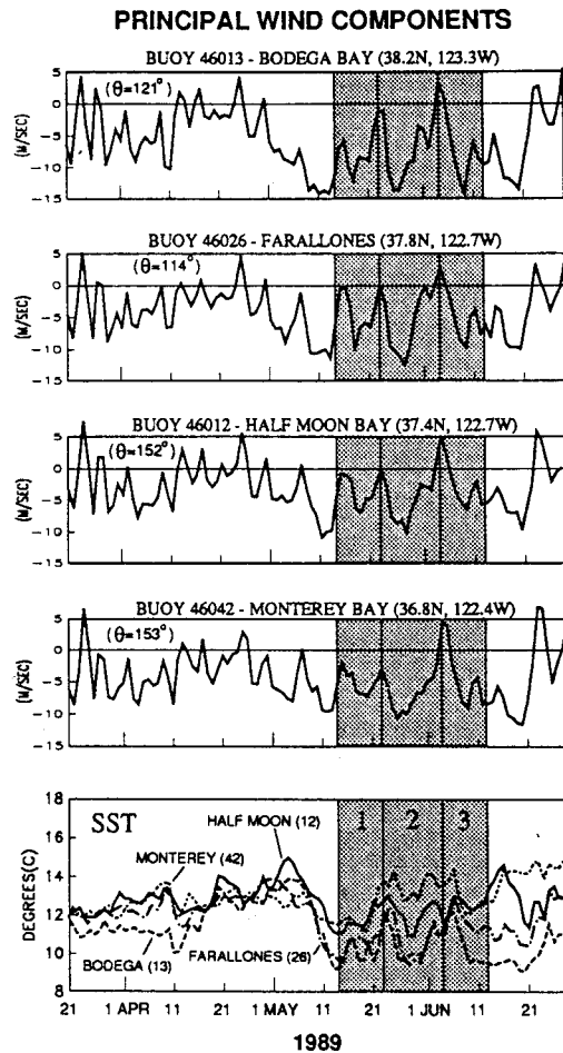
Figure 3. Time series of principal-axis wind component and sea-surface temperature (SST) from NDBC buoys for 21 March–29 June 1989. Negative wind speeds are in the direction of the principal axis, defined by \theta at each buoy. Shaded areas denote period of groundfish cruise.
