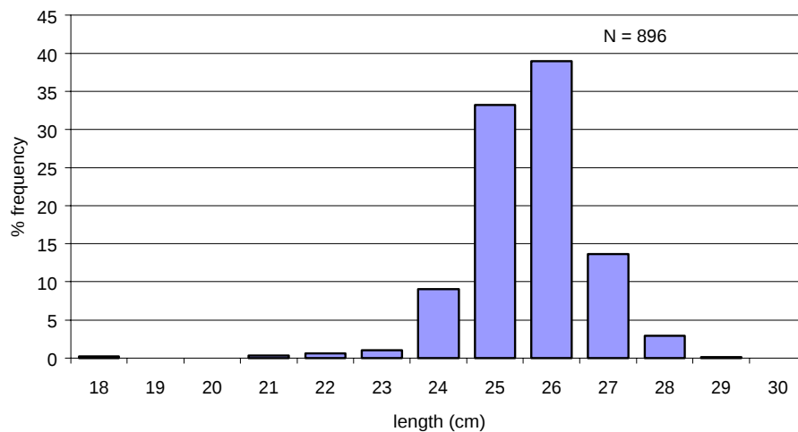
Figure 7. Length frequency for all sardines measured, August 6 – 19, 2003.
