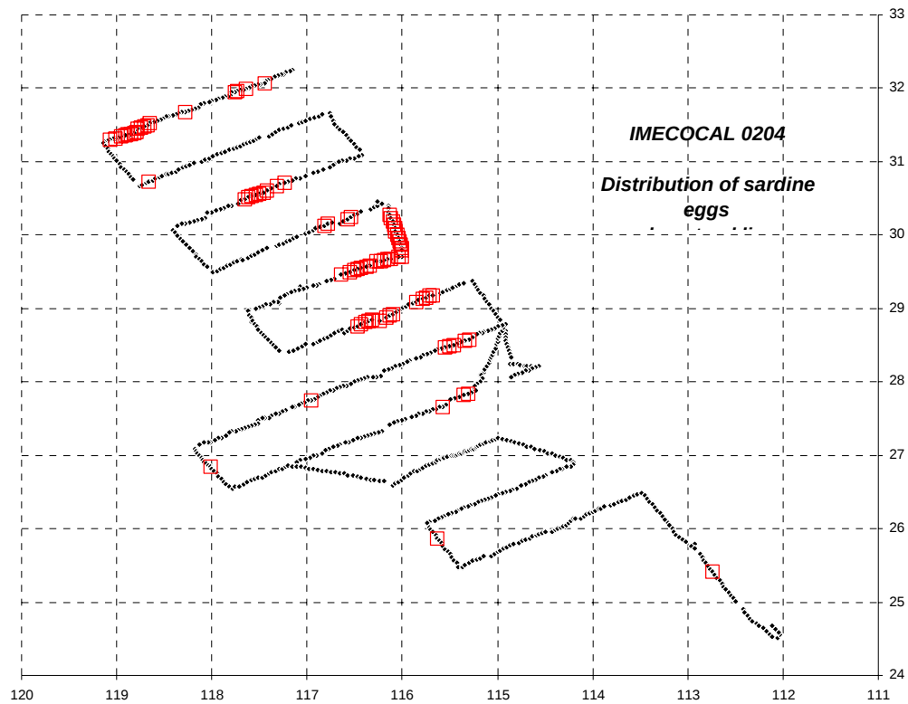
Figure 3. The distribution of eggs/min from CUFES collection during 0204 IMECOCAL survey. Red squares were positive for sardine eggs. Square denotes positive collection.
