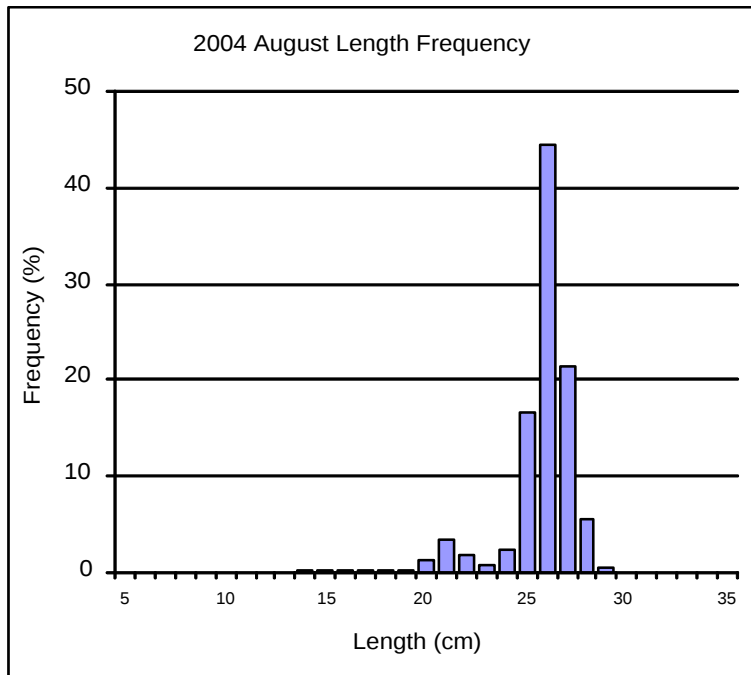
Figure 7a. Sardine length frequency during research cruise 2004-19.
