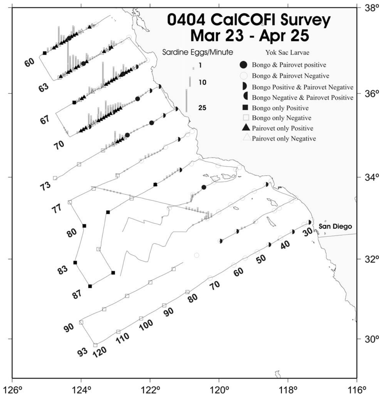
Figure 2. Sardine yolk-sac larvae from CalVET (or Pairovet; circle and triangle) and from Bongo (circle and square) in April 2004 survey. Solid symbols are positive and open symbols are zero catch.
