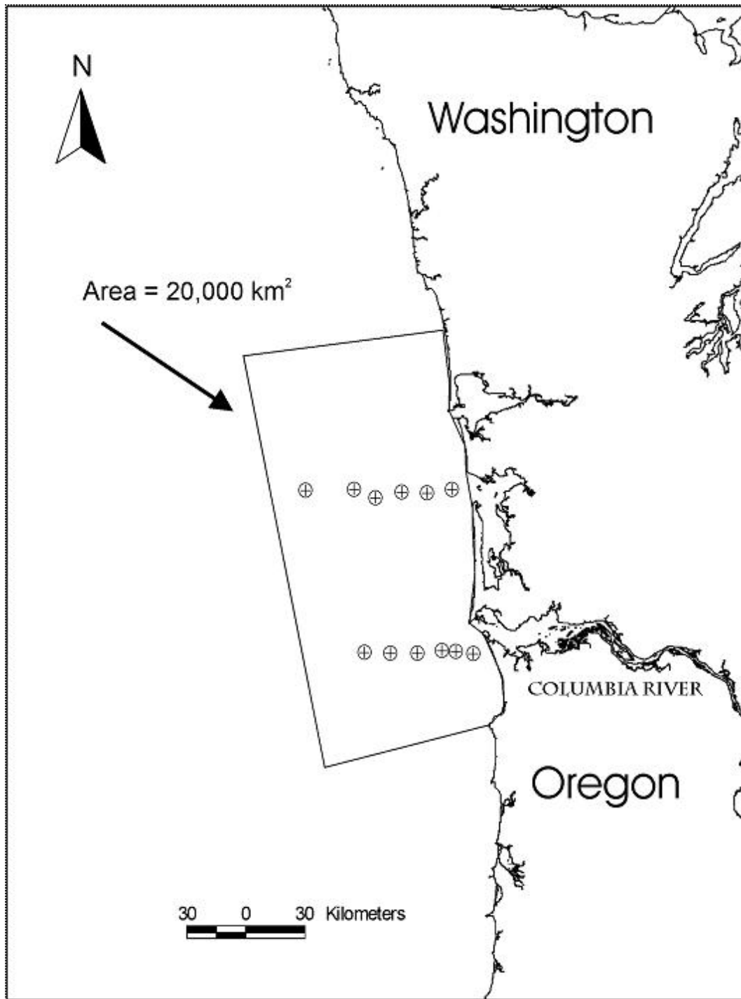
Figure 3. Survey area for Northwest surface trawl survey off Oregon and Washington from April-August, 2004.
