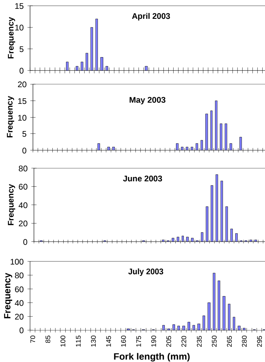
Figure 5. Distributions of fork length of Pacific sardine off Oregon and Washington, April-July, 2003
