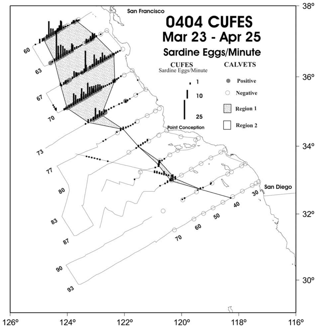
Figure 1. Sardine eggs from CalVET (or Pairovet; solid circle denotes positive catch and open circle denotes zero catch) and from CUFES (stick denotes positive collection) in April 2004 survey. The numbers on line 93 are CalCOFI station numbers. Region 1 is stippled area.
