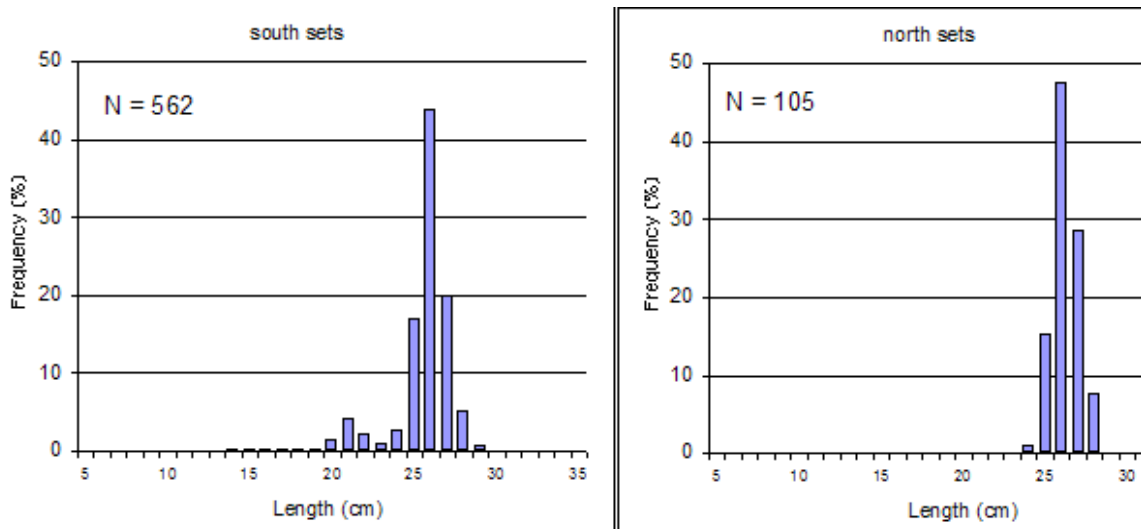
Figure 7b. Sardine length frequency by area during research cruise 2004-19.
