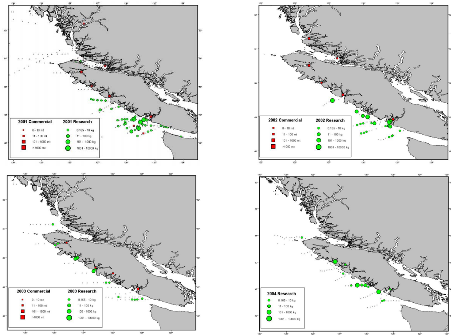
Figure 6. Distribution of relative abundance of sardine in trawl research surveys 2001-2004 off the west coast of Vancouver Island (Green = Research catch; Red = Commercial catch).
