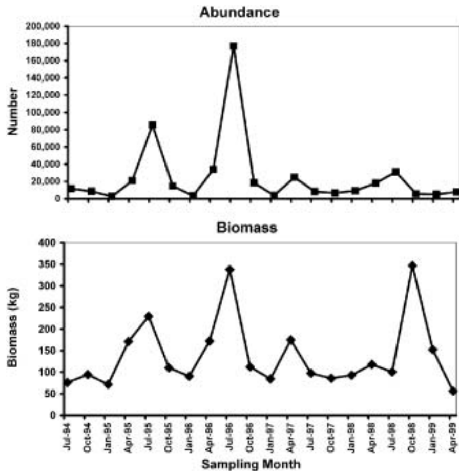
FIGURE 5-13 Seasonal variation in fish abundance (number) and biomass (kg) during a 5-year period in San Diego Bay (1994–1999) (after Allen et al., 2002).
