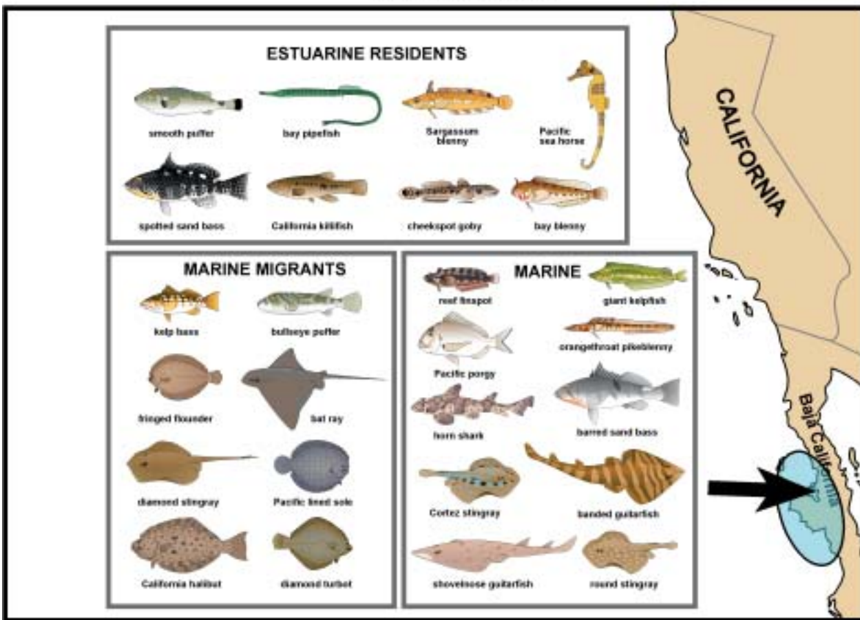
FIGURE 5-10 Profiles of fishes in Central Baja California bays and estuaries representing three ecological categories based on salt tolerance and life-history pattern: estuarine residents, marine migrants, and marine species that seasonally or occasionally enter these habitats. (See Table 5-3.)
