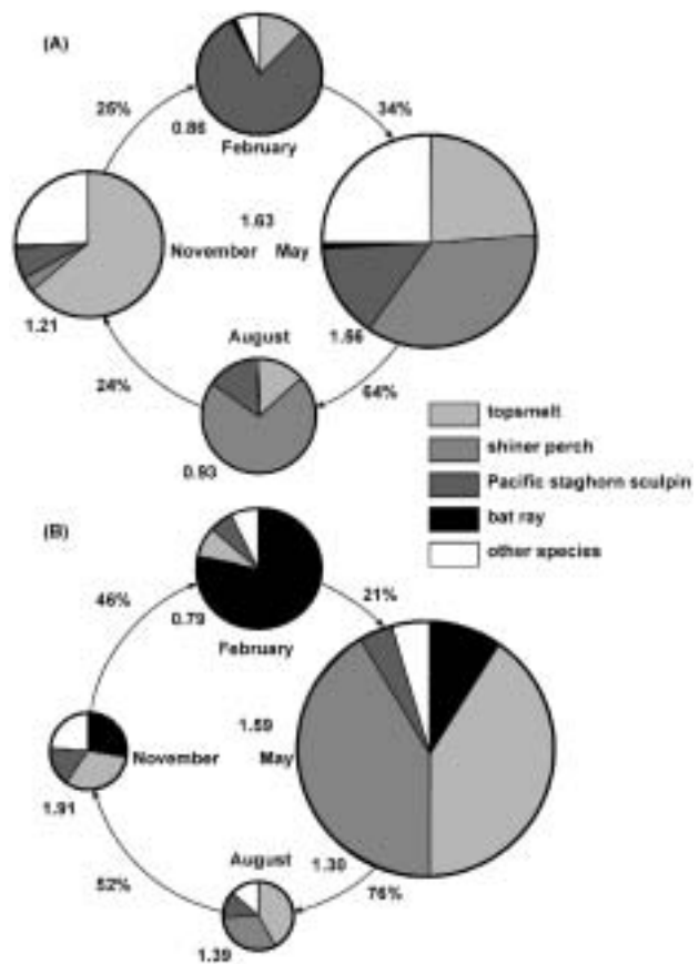
FIGURE 5-12 Seasonal pie diagrams depicting the annual cycle of (A) numbers and (B) biomass of four of the most common fish species and the remaining species collected by beach seine in the Baywood Park section of Morro Bay. Total diversity ( H' ) is given in the center of each cycle; the area of each circle is proportional to sample size, the number to the lower left of each circle is quarterly diversity H' , and the number on the connecting arrow is percentage similarity between months (after Horn, 1980).
