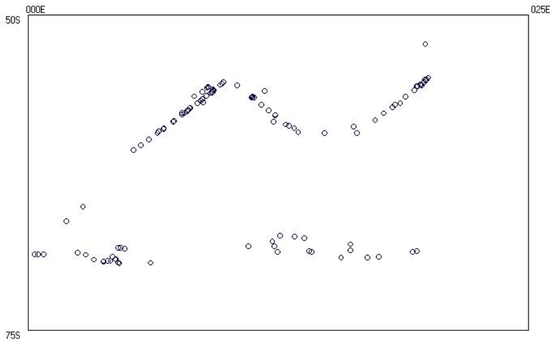
Figure 3a. Locations of all sonobuoy deployments during the cruise.
