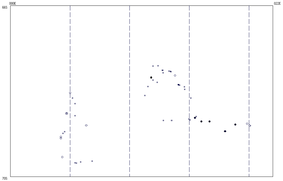
2e. Positions of sperm whale (□), killer whale (○) and southern bottlenose whale (●) observed in the minke whale research area.
