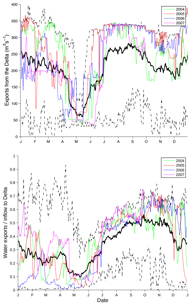
Figure 5: Daily export of freshwater from the delta (upper panel) and the ratio of exports to inflows (bottom panel). Heavy black line is the daily average discharge over the 1955-2007 period; dashed black lines indicate daily maximum and minimum discharges. Flow estimates from the DAYFLOW model ( http://www.iep.ca.gov/dayflow/ ).
