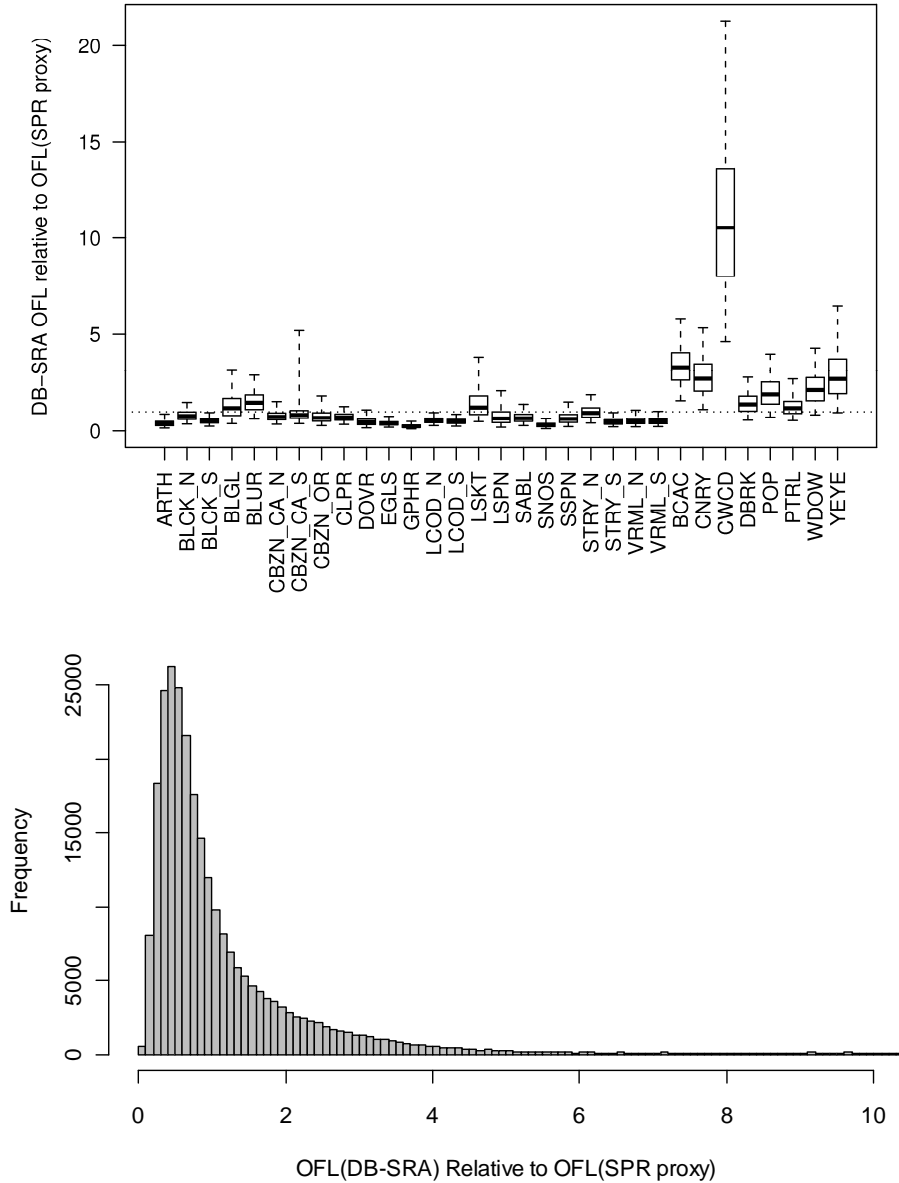
Figure 3. (Upper) DB-SRA estimates of OFL for 31 species, scaled relative to OFL(SPR proxy) estimates from the most recent assessment. Box-and-whisker plots characterize the median, IQR, and 95% intervals of the distributions. The reference line at unity represents agreement with the assessment’s point estimate. Uncertainty in the assessment estimate of OFL is not considered. (Lower): Distribution of OFL from DB-SRA, integrated across 31 stocks and scaled relative to the assessment estimates for OFL (SPR proxy). The upper tail is not fully displayed to better illustrate the dominant values of the distribution.
