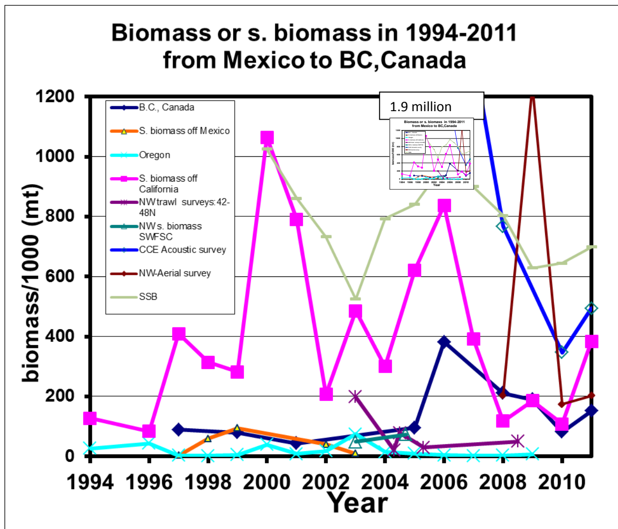
Figure 3: Time series of estimates of biomass and spawning biomass (s. biomass) from 1994-2011 from Mexico to British Columbia and spawning stock biomass (SSB) from 2011 stock assessment. Note the biomass estimate from the acoustic survey in 2006 was 1.9 million mt with large variance (Hunter and Baumgartner 2002; Lo and Allen 2008; Emmett and Lo 2009; Schweigert et al. 2010; Rodriguez-Sanchez et al. 2010; Hill et al. 2011).
