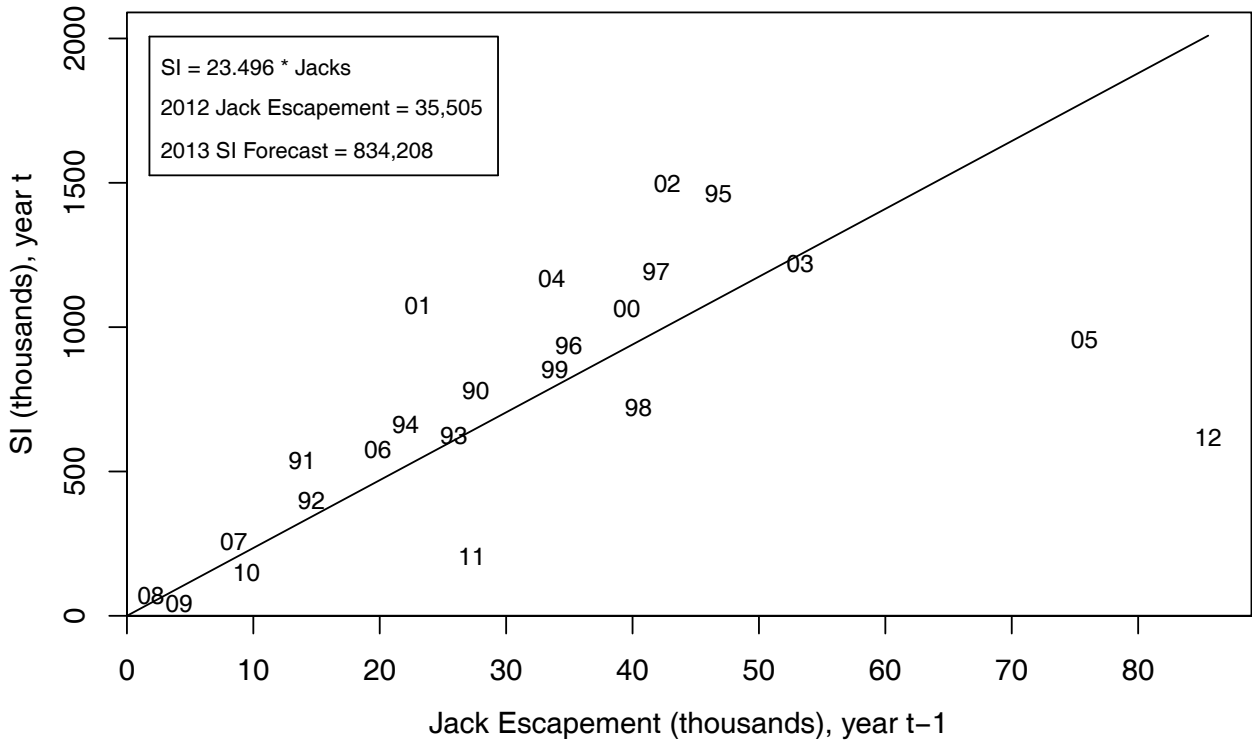
FIGURE II-2. Regression estimator for the SI based on previous year's escapement of Sacramento River fall Chinook jacks. Years shown are SI years.
