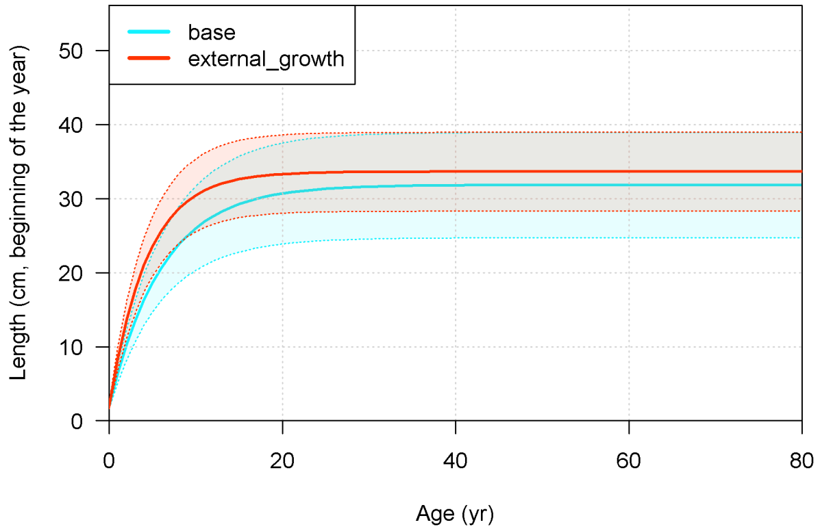
Figure 115: Sensitivity of the model to fixing growth parameters to external estimates in the southern model.
