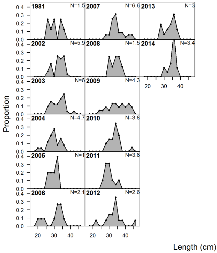
Figure 51: WDFW length compositions for the southern Washington recreational fleet, all modes.
