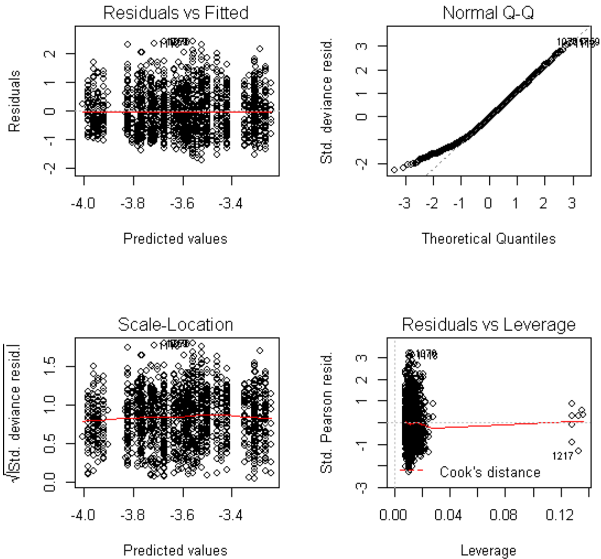
Figure 35: Diagnostic plots for the China rockfish delta-GLM index (lognormal component) for the Southern Oregon Recreational Boat Survey (ORBS) data set. These are used to evaluate model fit (top left), assumptions of normality (top right), assumptions of constant variance (bottom left), and the presence of outliers (bottom right).
