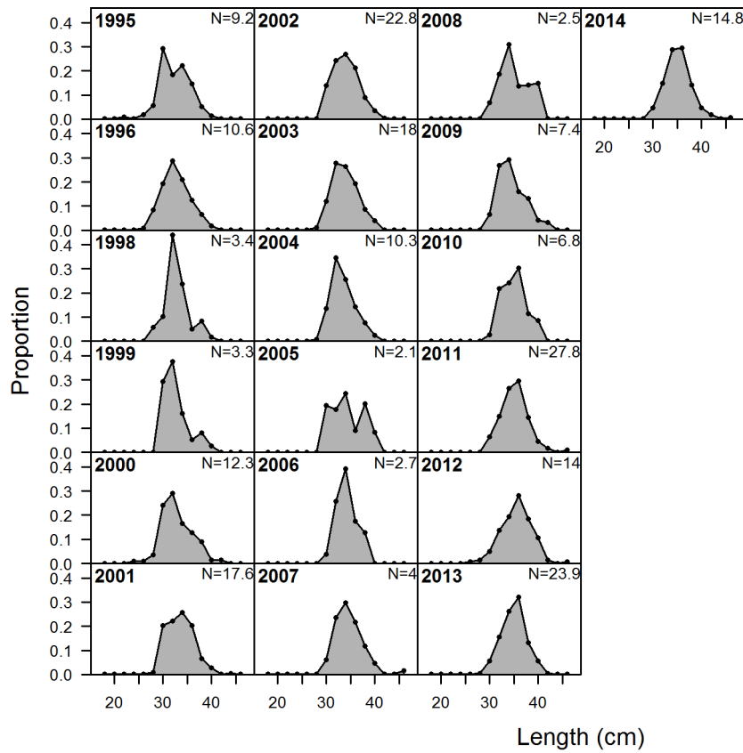
Figure 57: Length compositions for retained fish from the southern Oregon commercial dead-fish fishery.
