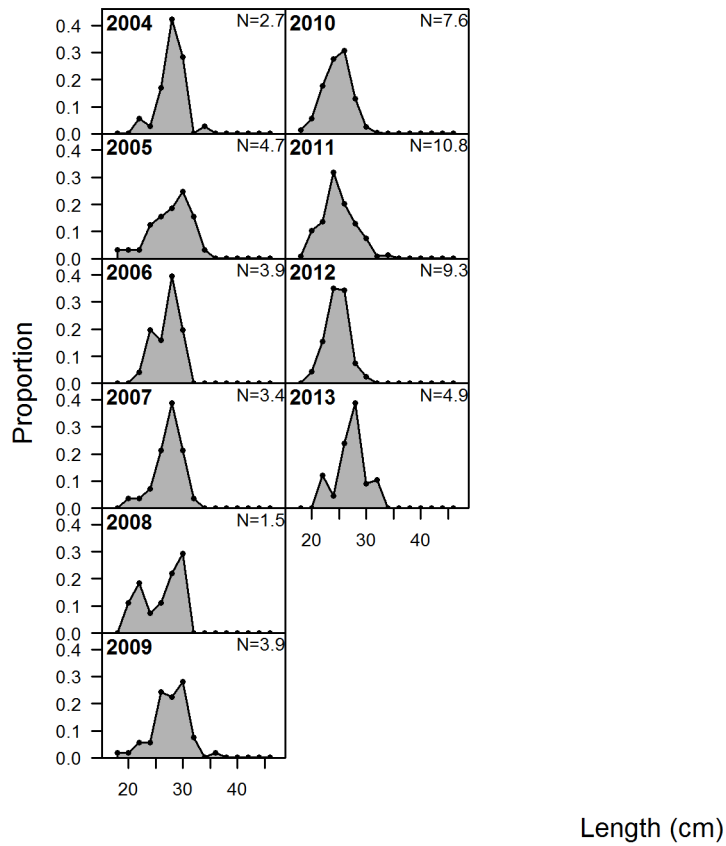
Figure 64: Length compositions by year for discarded fish in the California commercial fishery south of 40°10'.
