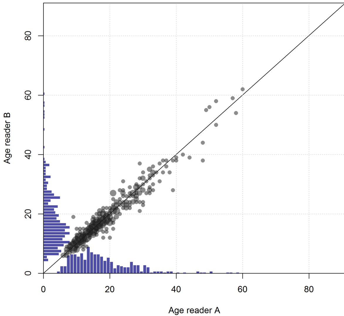
Figure 71: Aging precision between two current age readers at the NWFSC.
