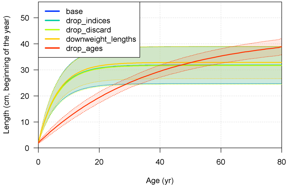
Figure 112: Sensitivity of removal of marginal age composition data and conditional age-at-length data from the southern model.
