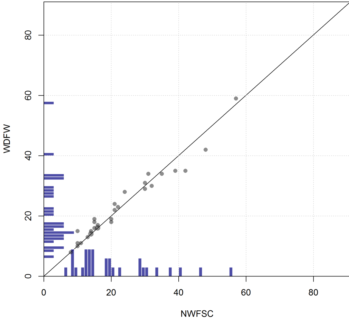
Figure 73: Aging precision between NWFSC and WDFW age readers.
