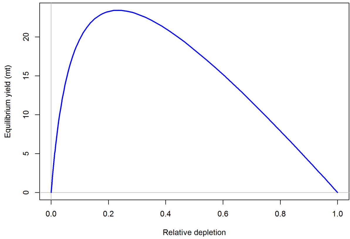
Figure 145: Equilibrium yield curve for the southern model.
