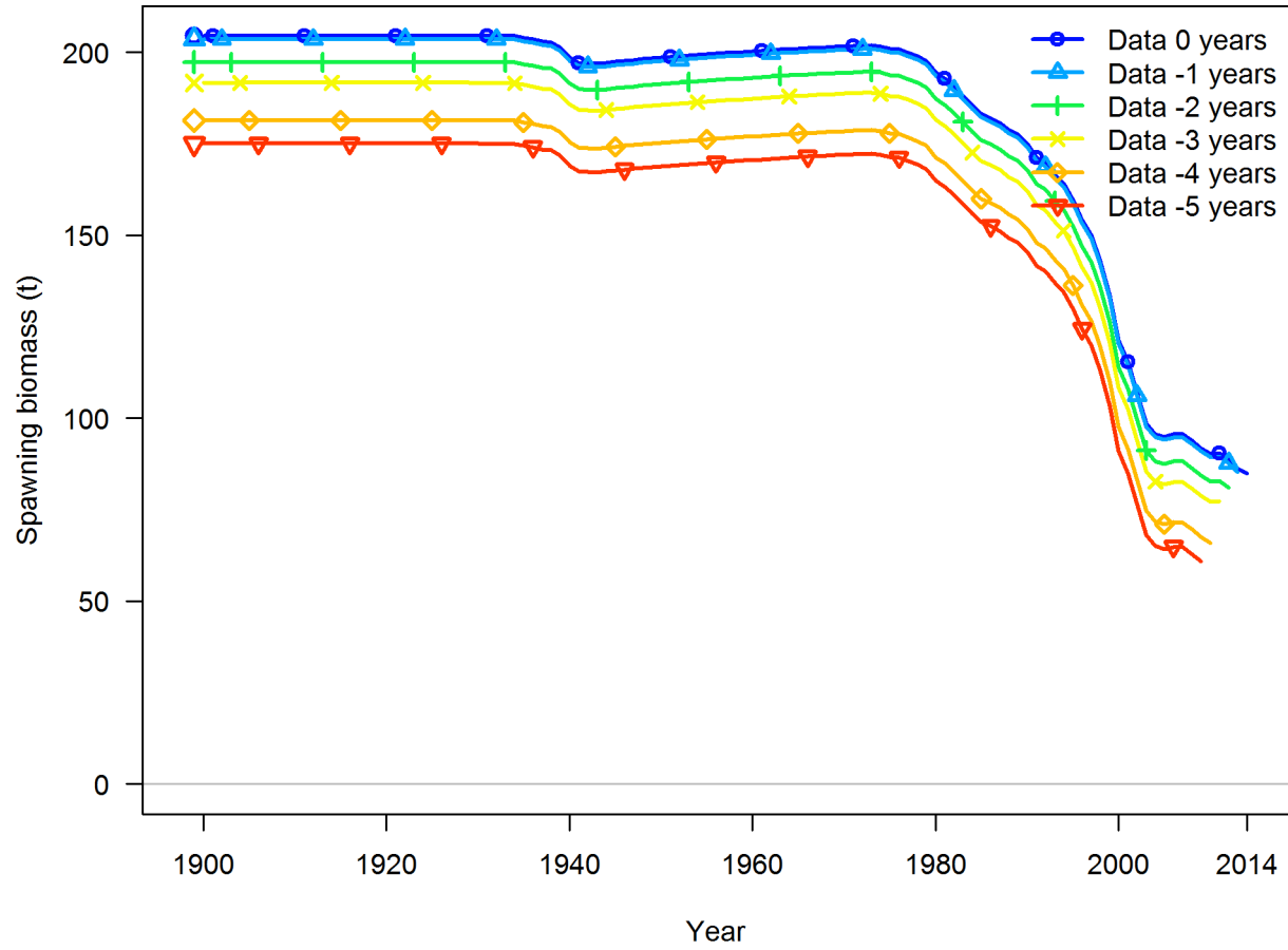
Figure 123: Retrospective analyses for the central model.
