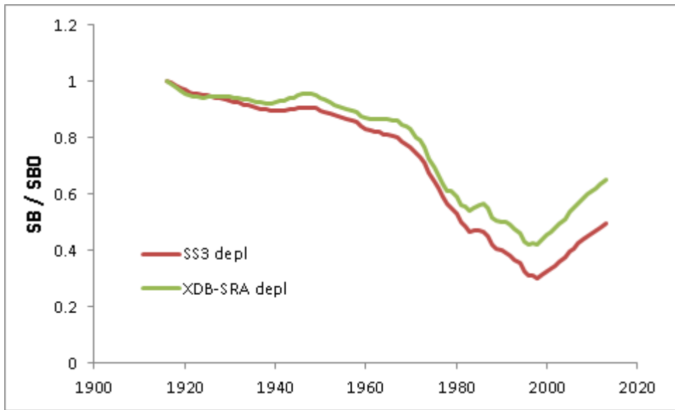
Figure 83: Time series of spawning biomass relative to unfished spawning biomass (“depletion”, or SB/SB0) from the 2013 XDB-SRA assessment of China rockfish south of 40°10' N. latitude, and an age-structured production model in Stock Synthesis v3 (SS3) fit to the same data.
