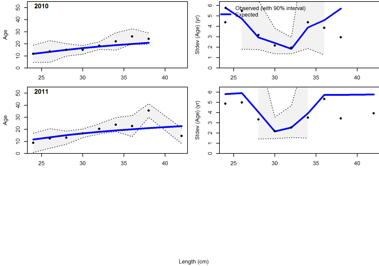
Figure 105: Fits to the conditional age-at-length data from Jeff Abrams' thesis, southern model.
