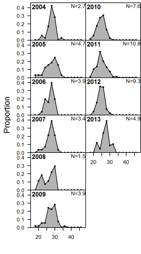
Figure 13: Length compositions by year for discarded fish in the California commercial fishery south of 40°10'.
