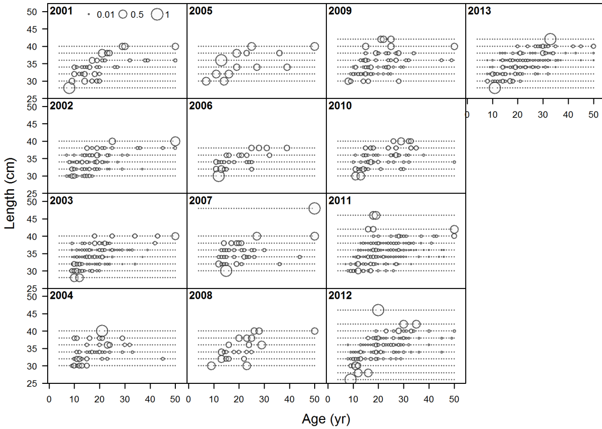
Figure 61: Conditional age-at-length data for retained fish from the southern Oregon commercial dead-fish fishery.
