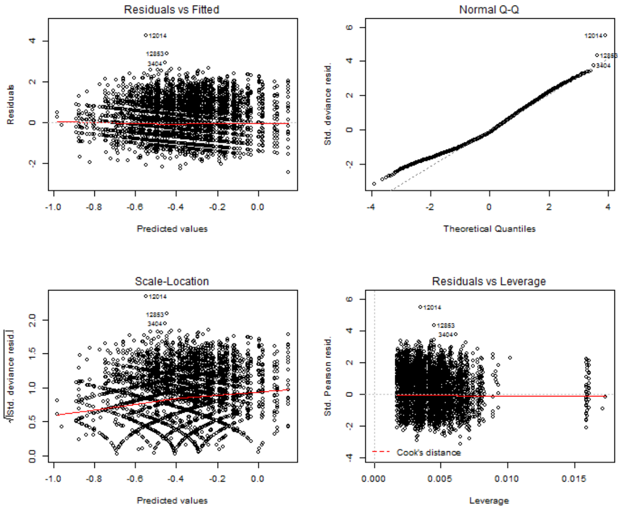
Figure 26: Diagnostic plots for the China rockfish positive catch component lognormal delta-GLM model for the dataset applying the Stephens-MacCall data filter, but retaining all of the positive records for the Washington dockside index. These are used to evaluate model fit (top left), assumptions of normality (top right), assumptions of constant variance (bottom left), and the presence of outliers (bottom right).
