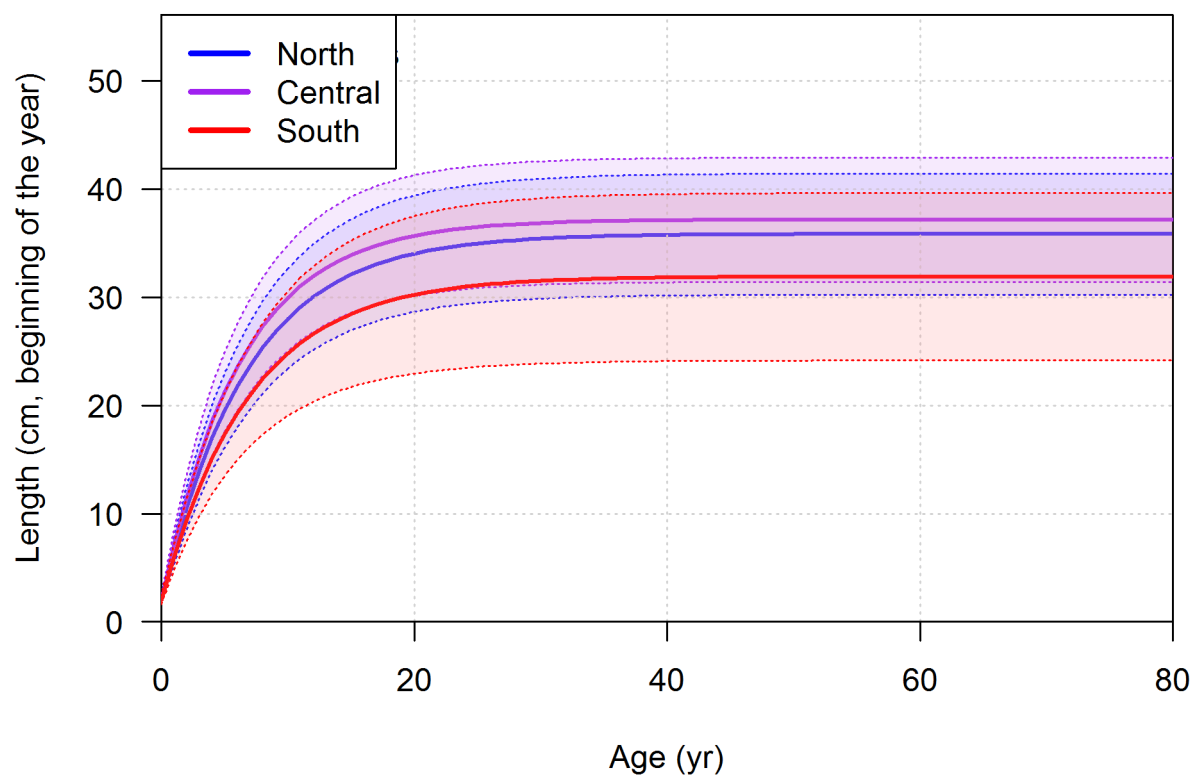
Figure 84: Fits to growth among models with no sex-specific growth.
