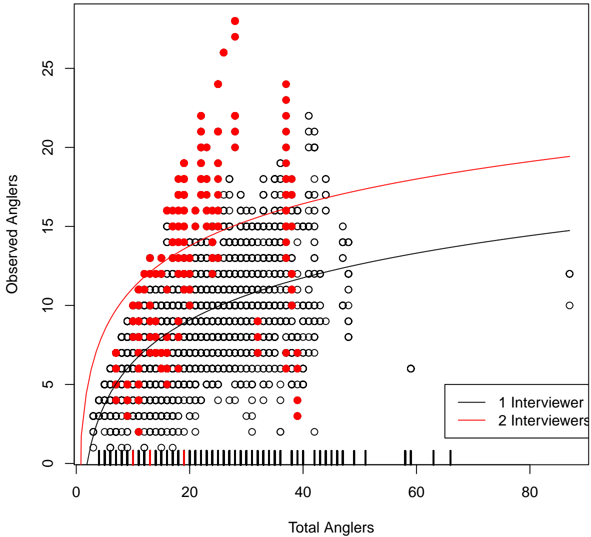
Figure E1: The number of observed anglers plotted as a function of the number of total anglers. The log-normal mean curves are plotted on the scale of the data, and colored to indicate if the data was collected in the presence of one or two interviewers. Additionally, a total anglers rug plot is included to show the total angler data for which the number of observed anglers needs to be imputed.
