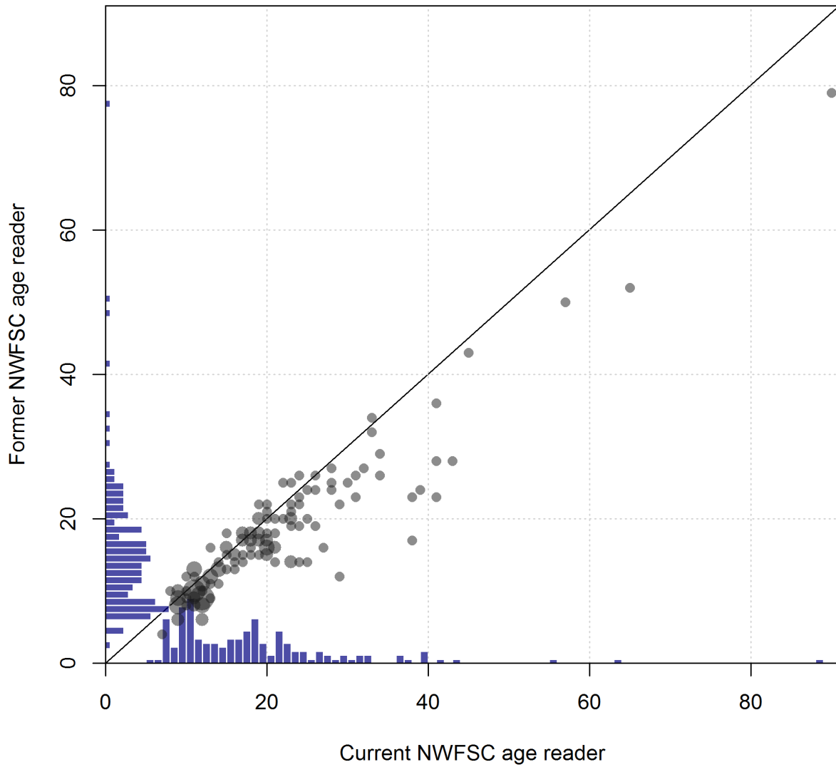
Figure 72: Aging precision between a current and former NWFSC age reader.
