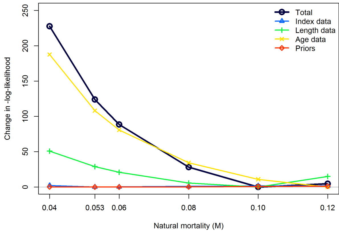
Figure 128: Likelihood profile over natural mortality, M , showing changes in negative log-likelihoods by data type for the pre-STAR central model.
