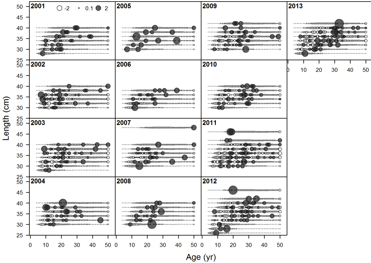
Figure 96: Residuals in fit to conditional age-at-length compositions for the commercial dead-fish fishery in southern OR in the central model. Filled circles indicate observed values greater than expected values.
