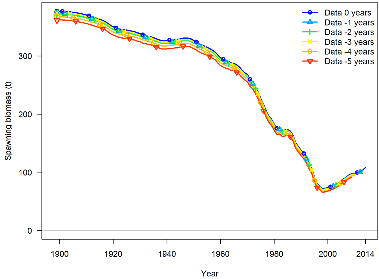
Figure 122: Retrospective analyses for the southern model.
