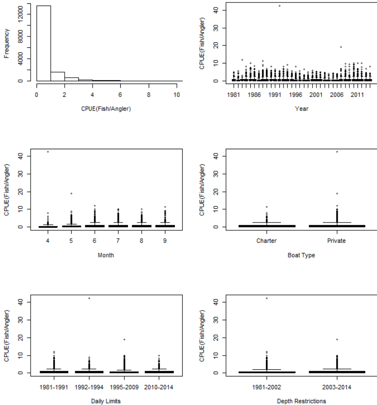
Figure 24: Summary data plots for the data set with Stephens-MacCall filtering for the Washington dockside index.
