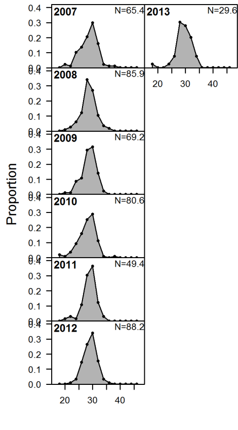
Figure 66: CCFRP research program length compositions for the southern model.
