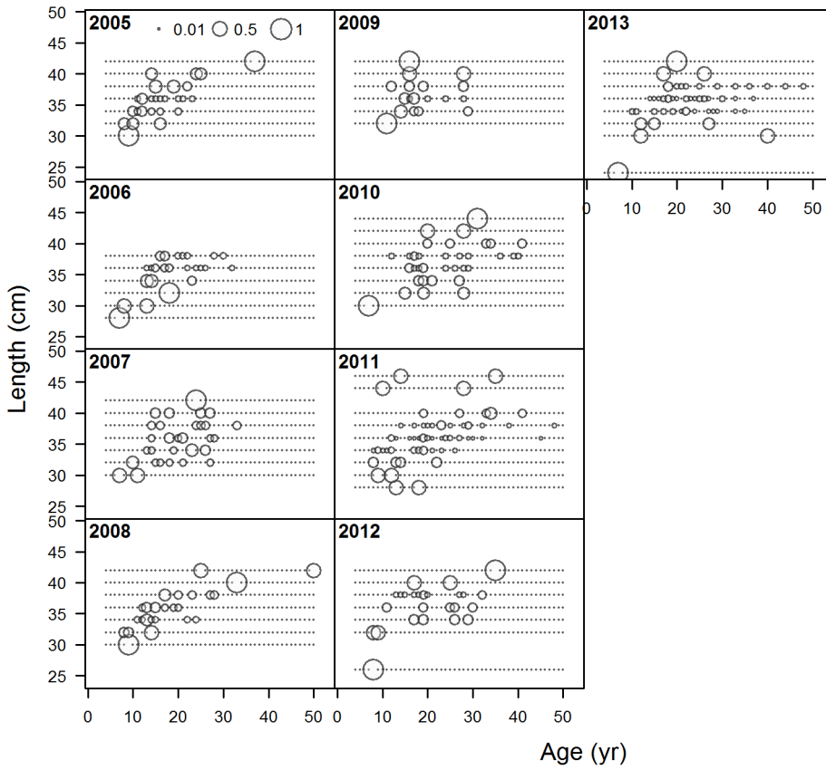
Figure 62: Conditional age-at-length compositions for the commercial dead-fish fishery in southern OR in the central model.
