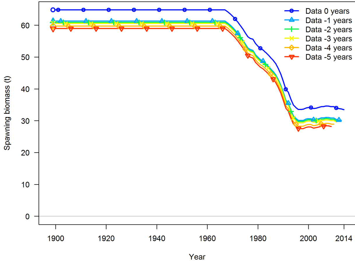
Figure 124: Retrospective analyses for the northern model.
