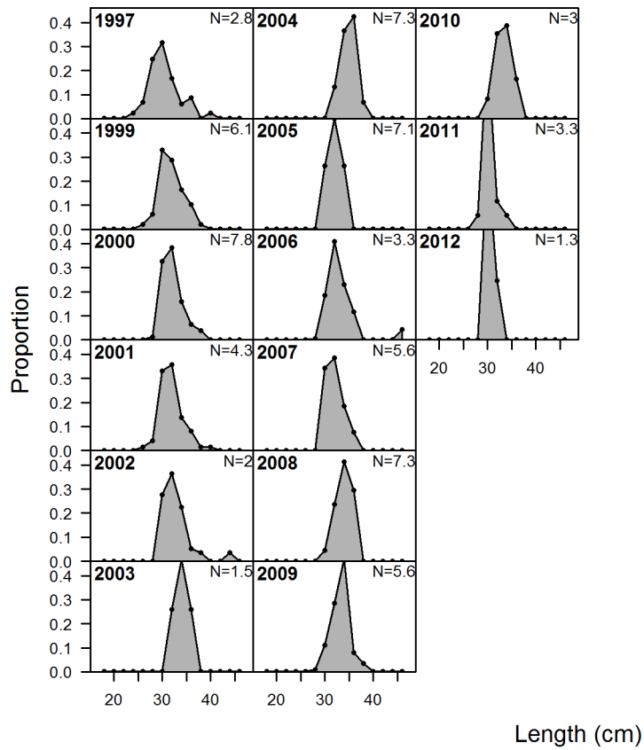
Figure 65: Length compositions by year for retained fish in the California commercial live-fish fishery south of 40°10'.
