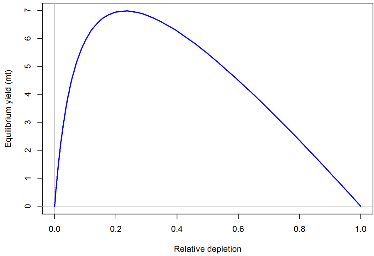
Figure 139: Equilibrium yield curve for the northern model.
