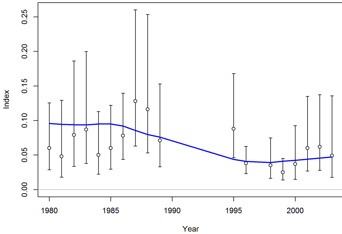
Figure 100: Fits to the CA recreational CPFV fleet dockside index for the southern model.
