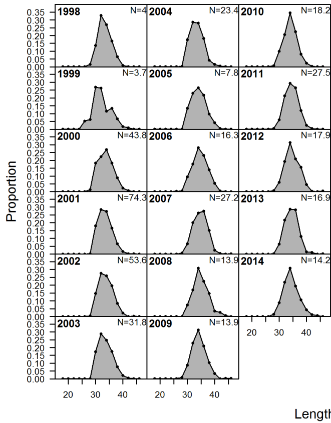
Figure 58: Length compositions for retained fish from the southern Oregon commercial live-fish fishery.
