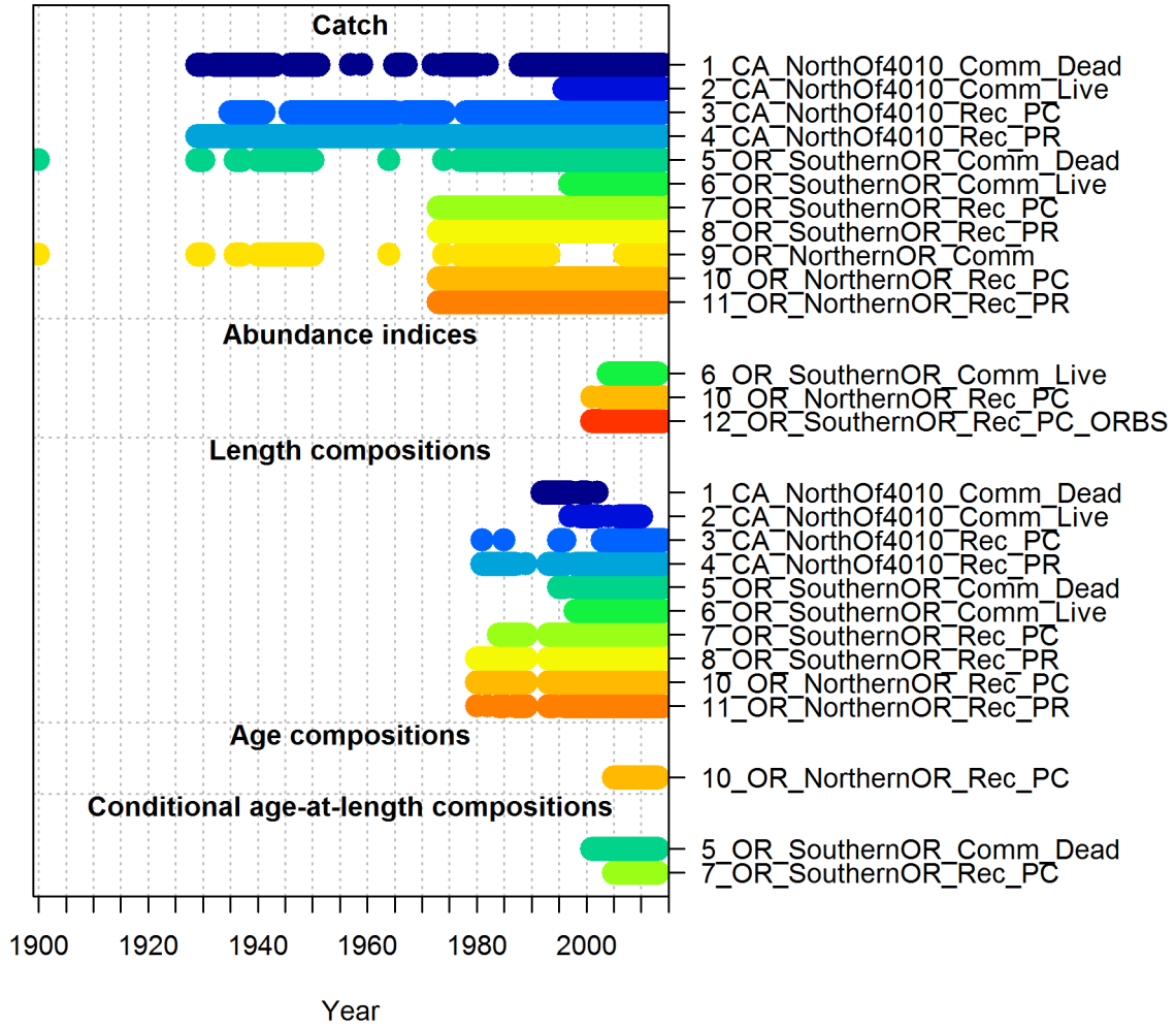
Figure 3: Summary of data sources used in the central assessment.
