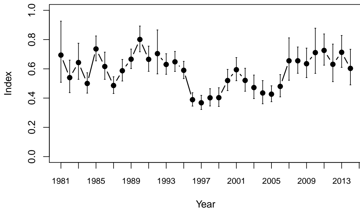
Figure 29: Index for the Washington dockside program, with 95% lognormal confidence intervals, applying the Stephens-MacCall data filter and retaining all positive observations.
