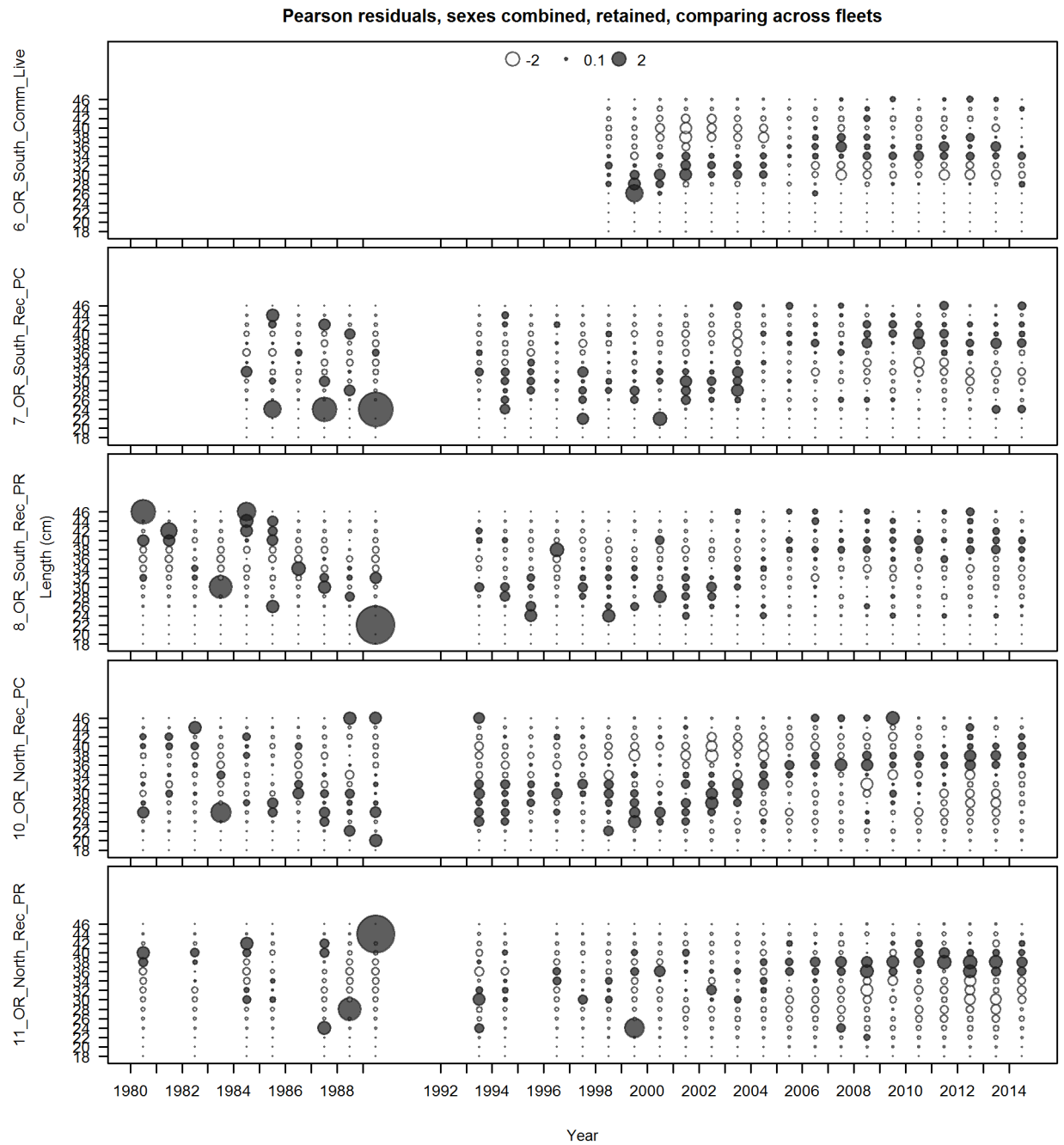
Figure 95: Residuals in fit to length compositions for northern model. Filled circles indicate observed values greater than expected values continued, figure 2 of 2.
