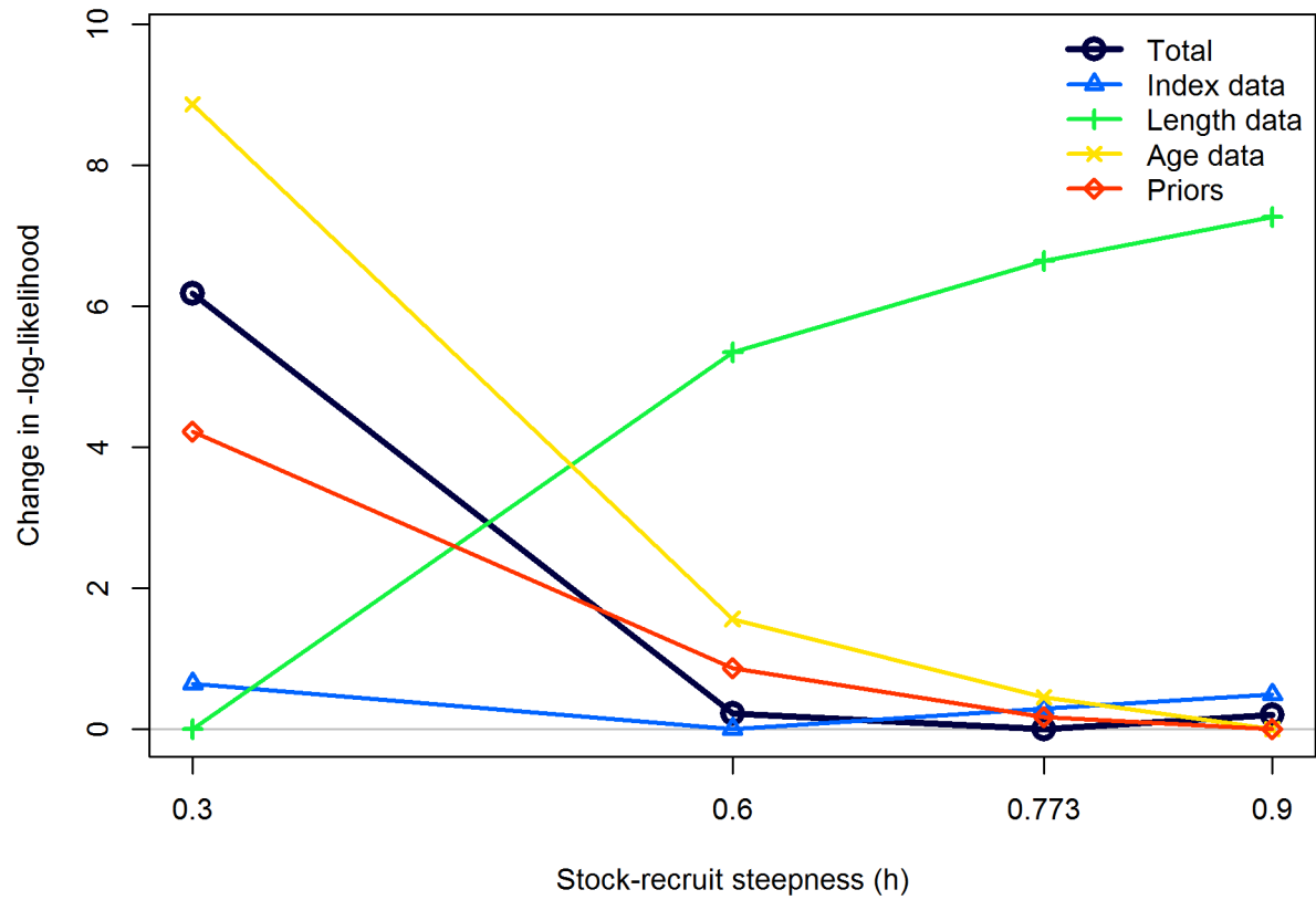
Figure 133: Likelihood profile over the steepness of the stock-recruit relationship, h , showing changes in negative log-likelihoods by data type for the pre-STAR central model.
