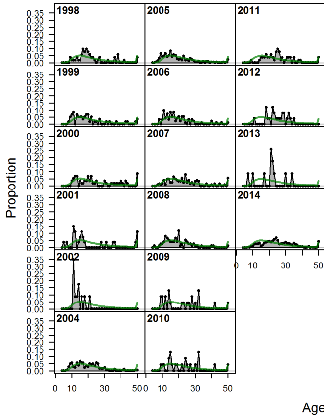
Figure 89: Implied fit to the marginal age-frequencies for recreational private/rental catch in northern WA in the northern model. Fits are provided for evaluation only, but not included in the model likelihood as these samples are included in the likelihood as conditional-age-at-length data.
