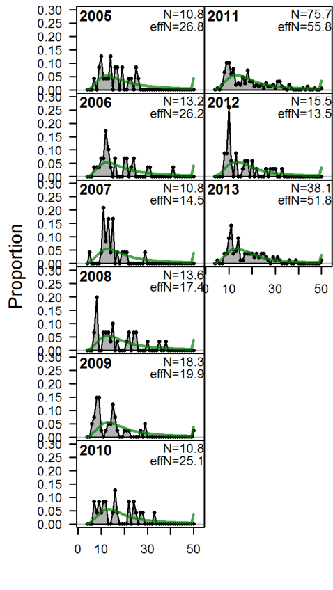
Figure 98: Fits to the marginal age composition for the northern OR recreational party/charter in the central model
