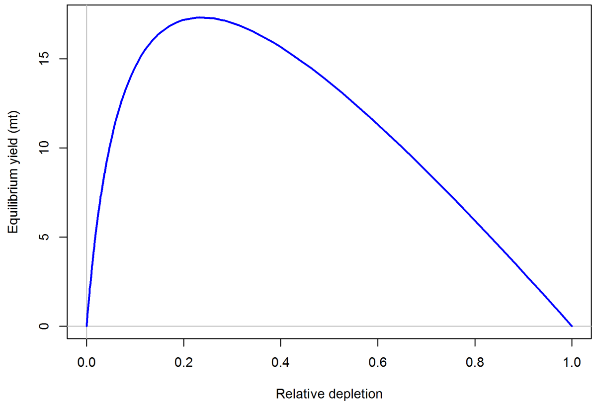
Figure 142: Equilibrium yield curve for the central model.
