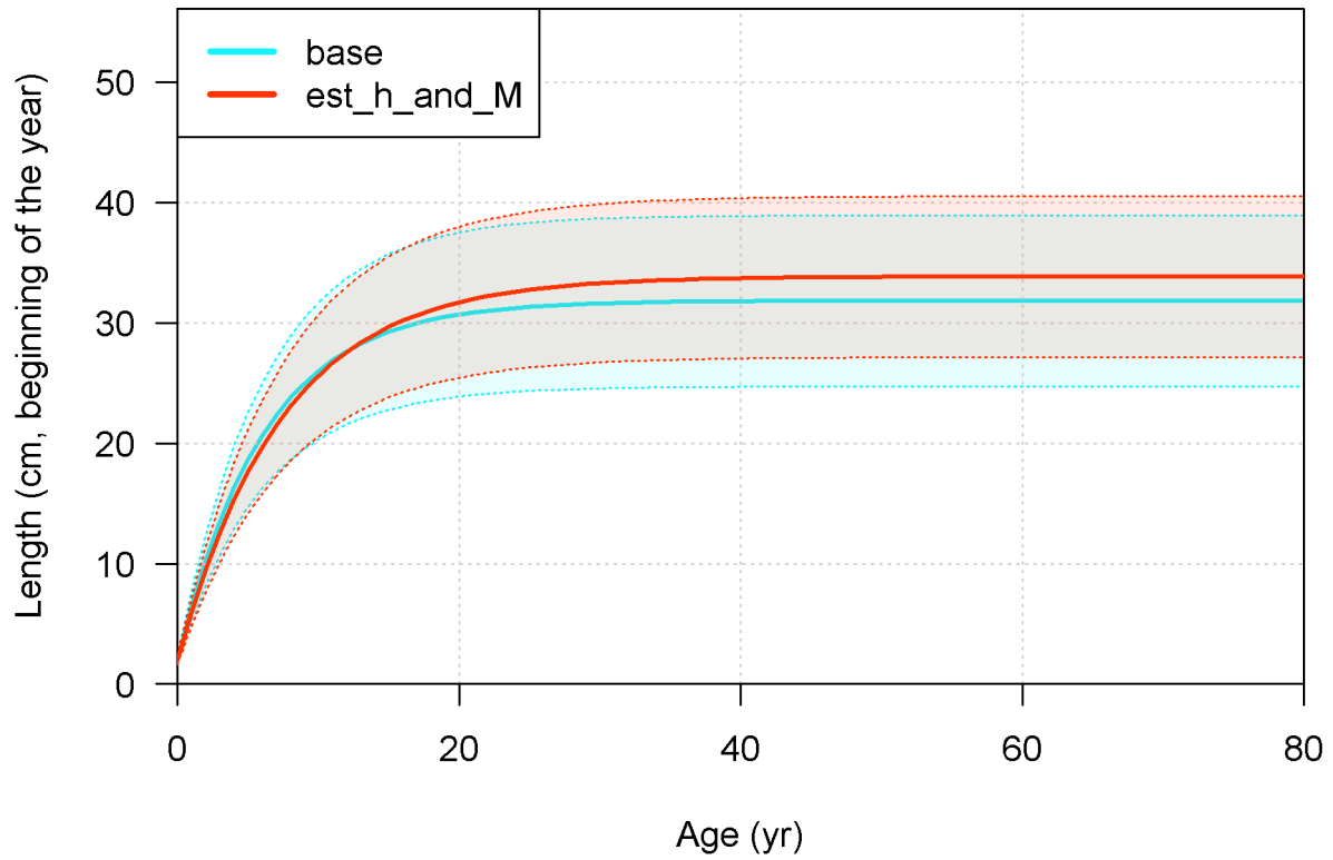
Figure 121: Sensitivity of growth to fixed versus estimated values of steepness and natural mortality to estimated values in the southern model.
