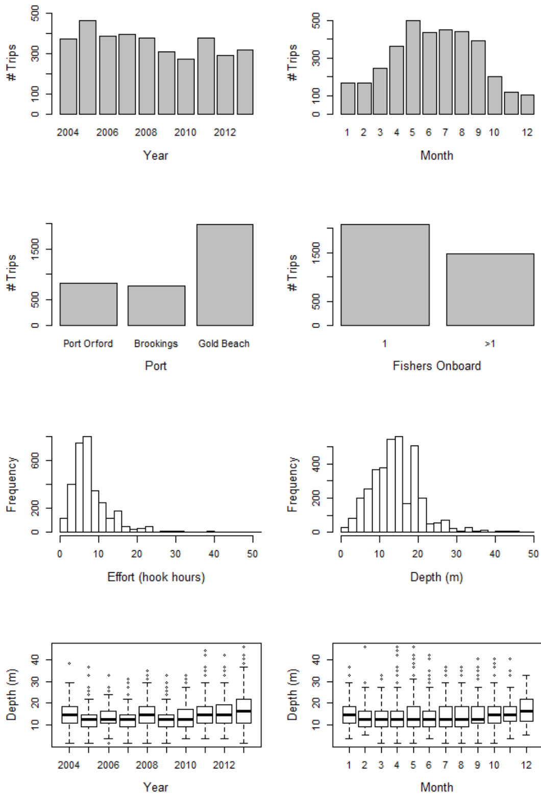
Figure 20: Characterization of the final subset of Oregon commercial logbook data used in delta-GLM analyses for China rockfish. 165
