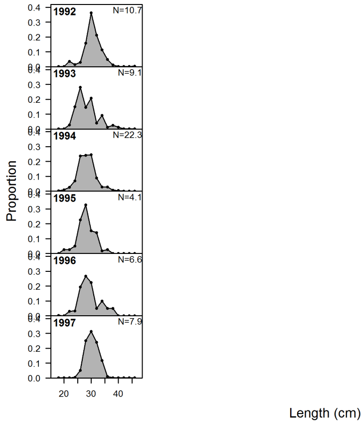
Figure 63: Length compositions by year for the California commercial dead-fish fishery south of 40°10'.
