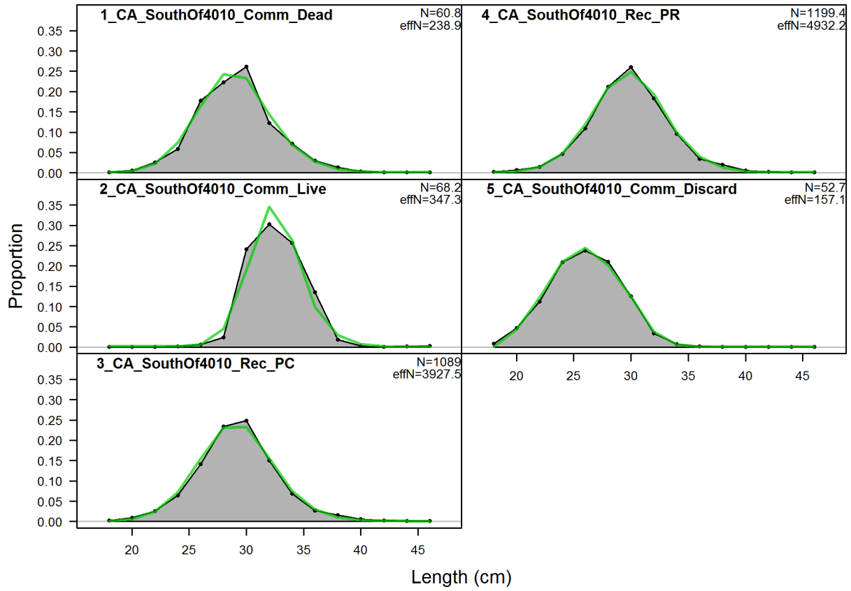
Figure 103: Fits to the length compositions from fleets in the southern model.
