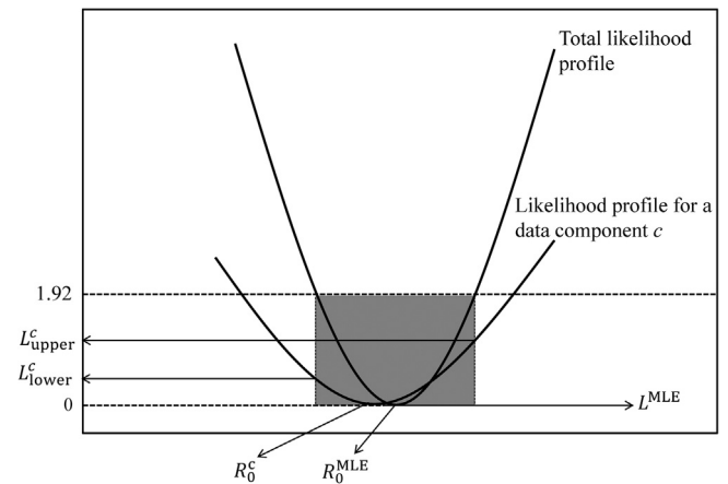
Fig. 4. Calculation of the R 0 component likelihood profile statistic. The grey area represents the 95% confidence interval for R 0 .
