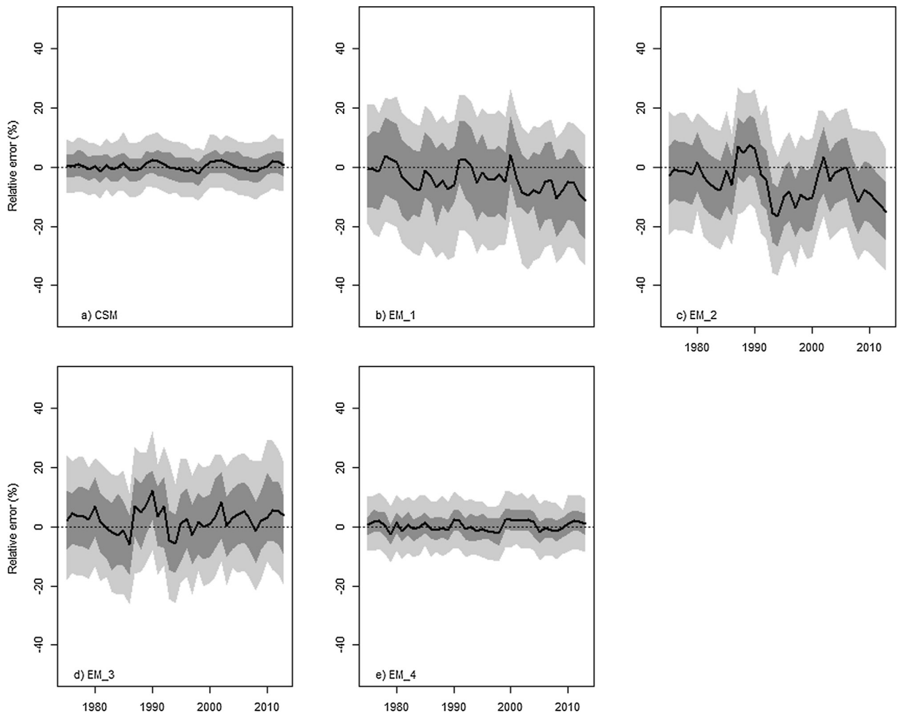
Fig. 6. Relative error distributions (median relative errors, and 50% and 90% intervals) for the time-trajectory of spawning stock biomass of WCNP striped marlin.
