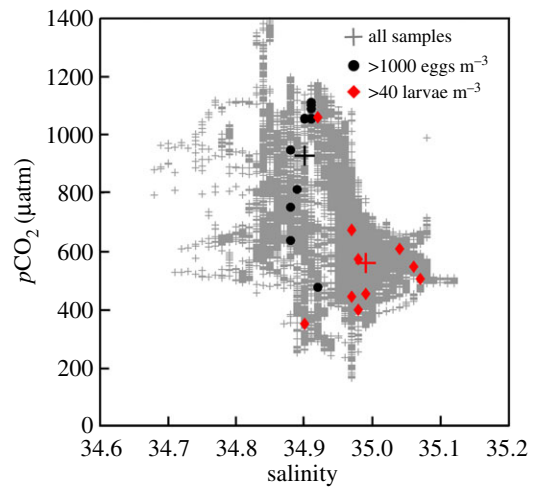
Figure 2. p\text{CO}_2 -salinity diagram for all seawater measurements (grey plus signs), CUFES samples containing more than 1000 eggs \text{m}^{-3} (black circles) and samples of larvae containing more than 40 larvae \text{m}^{-3} (red diamonds). The centroids of the distributions are indicated by the black and red plus signs.
