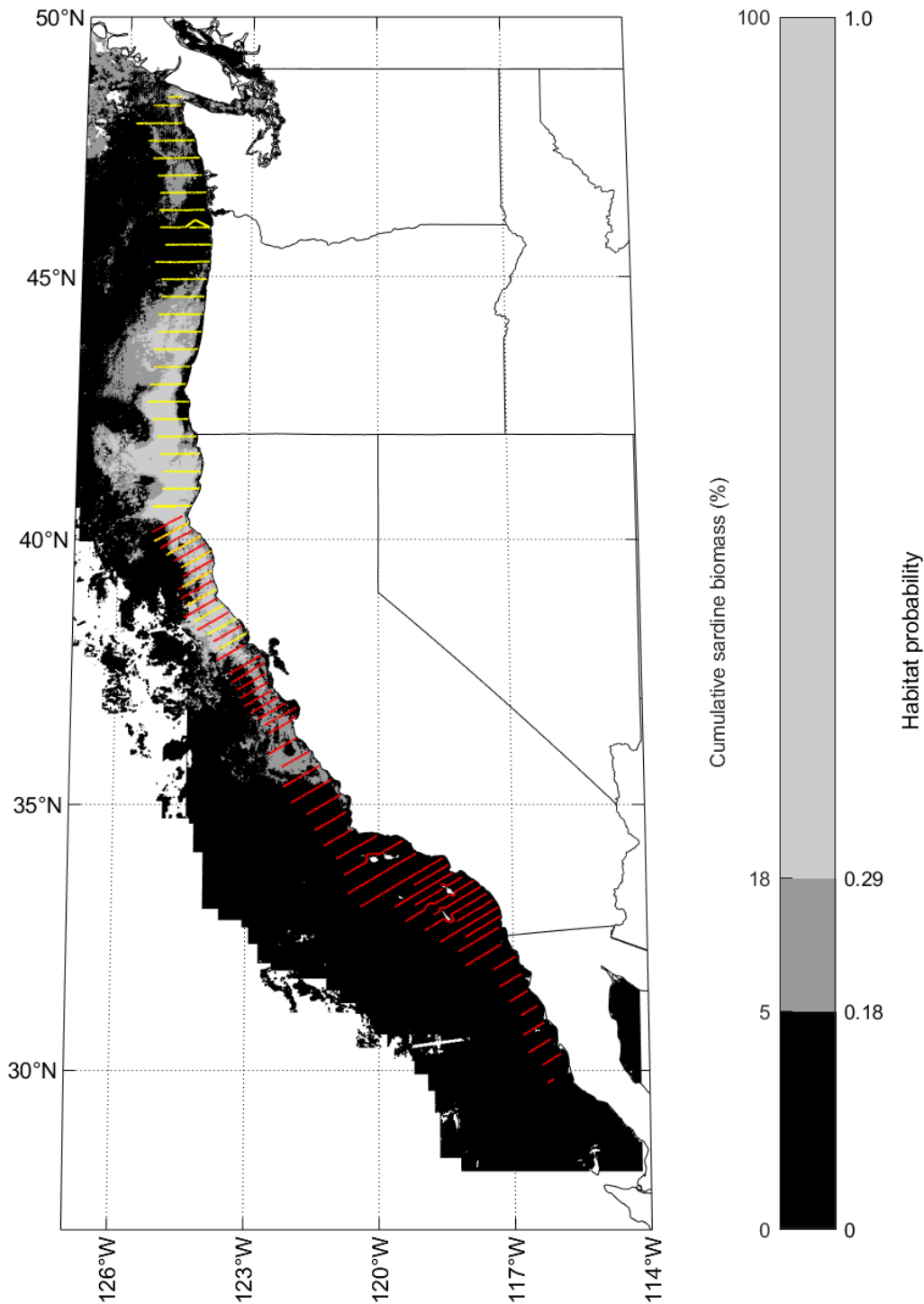
Figure 12: Summary of all transects sampled throughout the survey by Lasker (red) and Lisa Marie (yellow) in relation to the probability thresholds of the revised model of potential habitat for the northern stock of Pacific Sardine (Zwolinski and Demer, In prep.). The shaded regions with probabilities higher than 0.29 and 0.18 contained 82% and 95% of all spring northern stock Pacific Sardine spawning stock biomass, respectively. The habitat-model output is averaged in areas, \pm 2^\circ latitude and longitude, centered around the daytime location of each vessel throughout the survey. Areas without data (white), occurred in the analysis domain where and when clouds prevented satellite-sensed observations.
