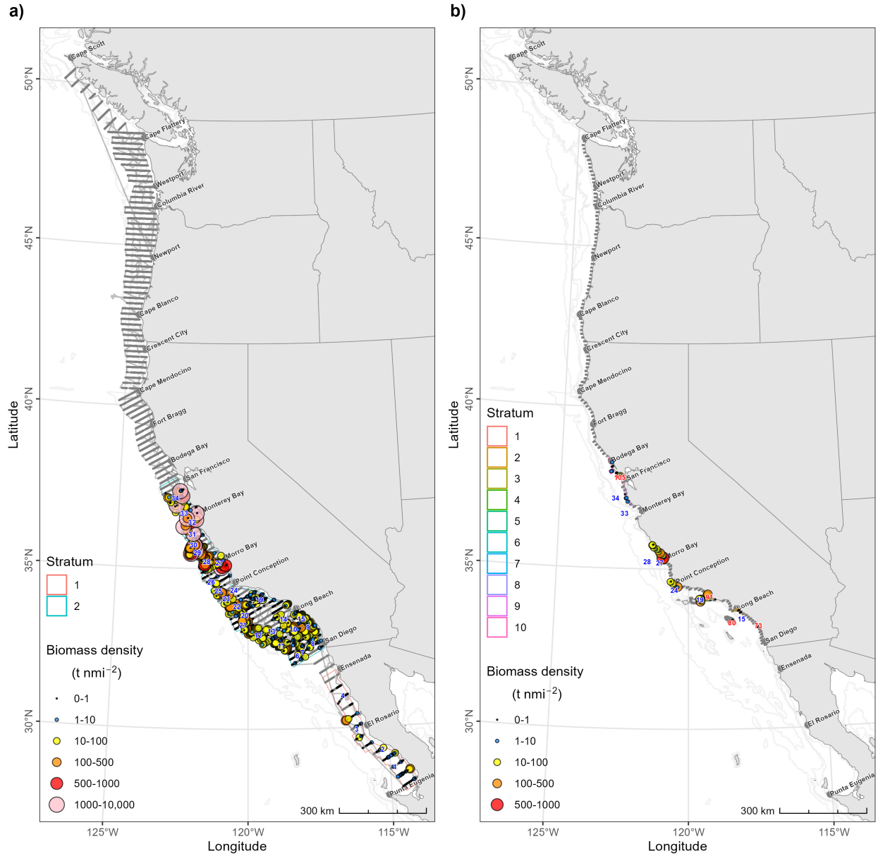
Figure 22: Biomass densities (colored points) of central subpopulation of Northern Anchovy ( Engraulis mordax ), per stratum, in the a) core and b) nearshore survey regions. Overlaid are the locations of trawl clusters (blue numbers) or purse seine samples (red numbers) with at least one Northern Anchovy in each stratum (colored polygons). Thick gray lines represent acoustic transects.
