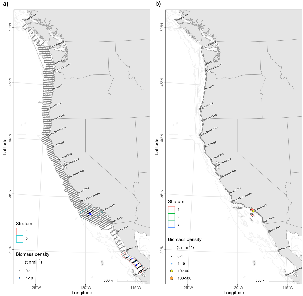
Figure 34: Biomass densities (colored points) of Round Herring ( Etrumeus acuminatus ), per stratum, in the a) core and b) nearshore survey regions. Overlaid are the locations of trawl clusters (blue numbers) or purse seine samples (red numbers) with at least one Round Herring in each stratum (colored polygons). Thick gray lines represent acoustic transects.
