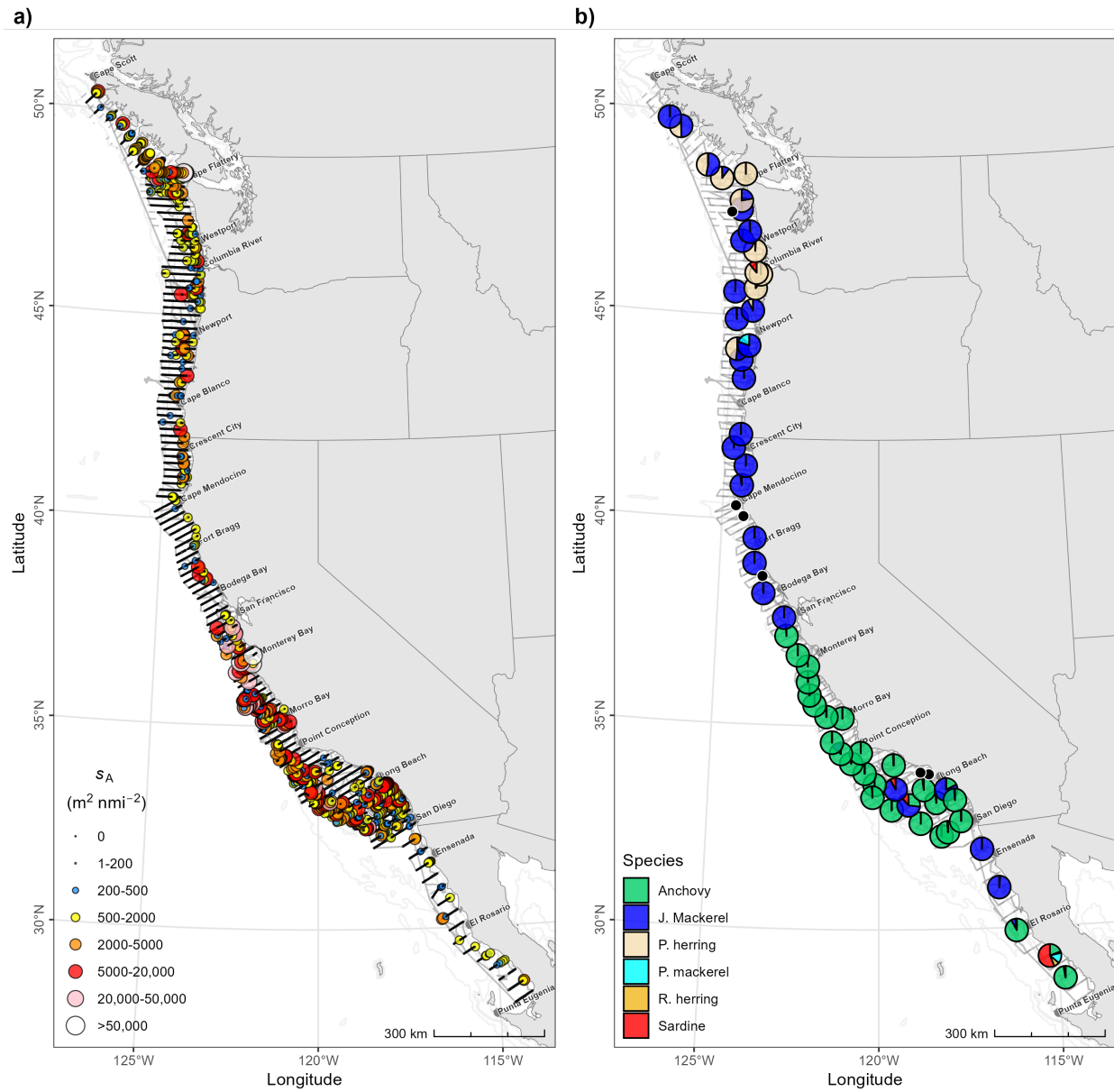
Figure 17: Spatial distributions of: a) 38-kHz vertically integrated backscattering coefficients ( s_A , \text{m}^2 \text{nmi}^{-2} ; averaged over 2000-m distance intervals) ascribed to CPS and b) proportion of acoustic backscatter from CPS in trawl clusters sampled by Lasker .
