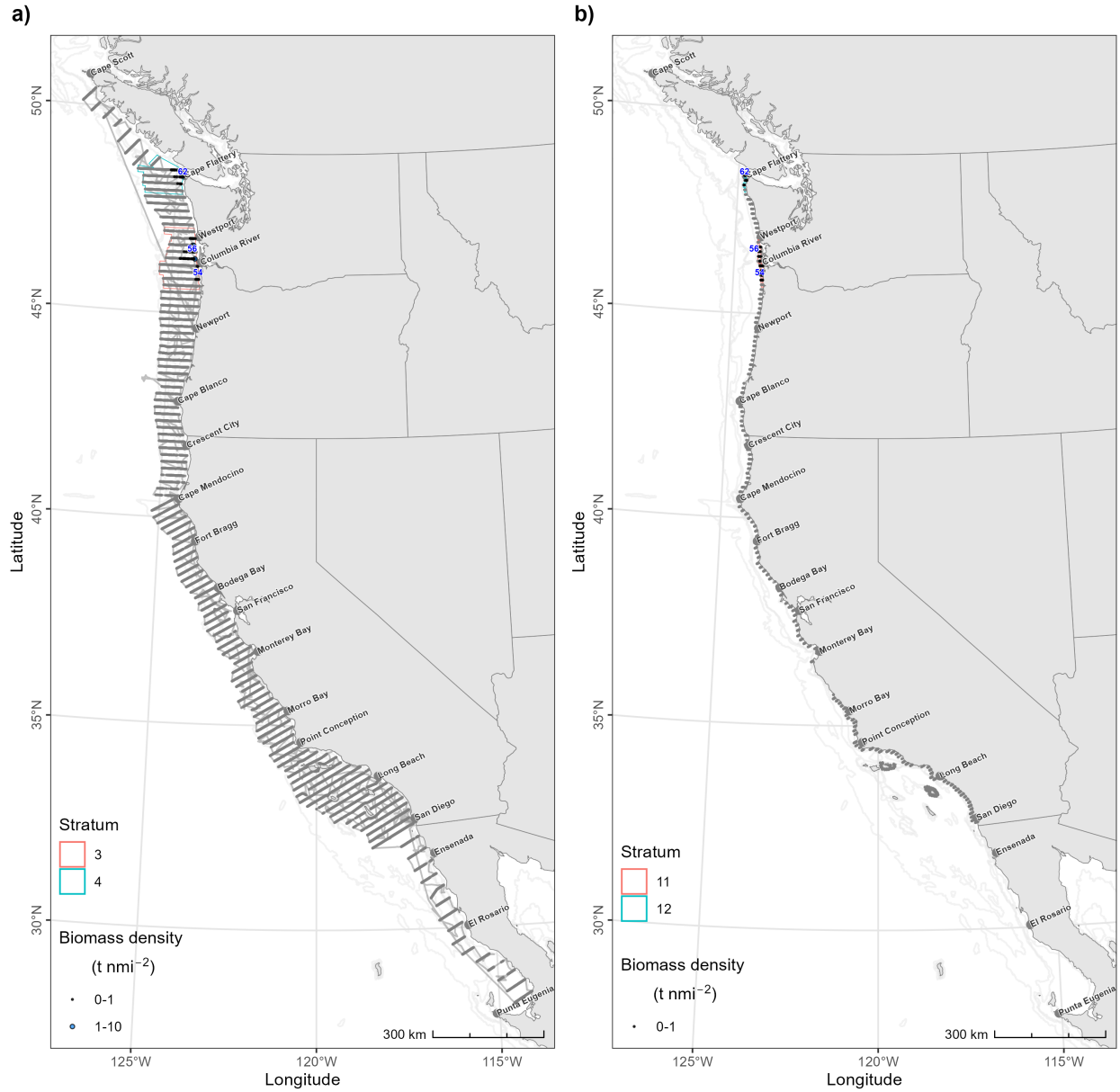
Figure 20: Biomass densities (colored points) of the northern subpopulation of Northern Anchovy ( Engraulis mordax ), per stratum, in the a) core and b) nearshore survey regions. Overlaid are the locations of trawl clusters (blue numbers) or purse seine samples (red numbers) with at least one Northern Anchovy in each stratum (colored polygons). Thick gray lines represent acoustic transects.
