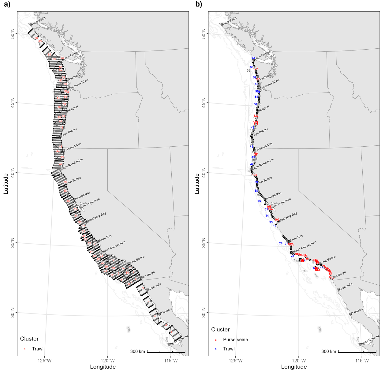
Figure 13: Polygons enclosing 100 m-long acoustic transect intervals sampled by a) Lasker in the core region and b) Long Beach Carnage and Lisa Marie in the nearshore region relative to the nearest trawl cluster or purse-seine set used to apportion acoustic backscatter. The colored numbers inside each polygon indicate the sample number and gear type. Dark gray numbers indicate trawl clusters or purse-seine sets with no CPS present in the catch.
