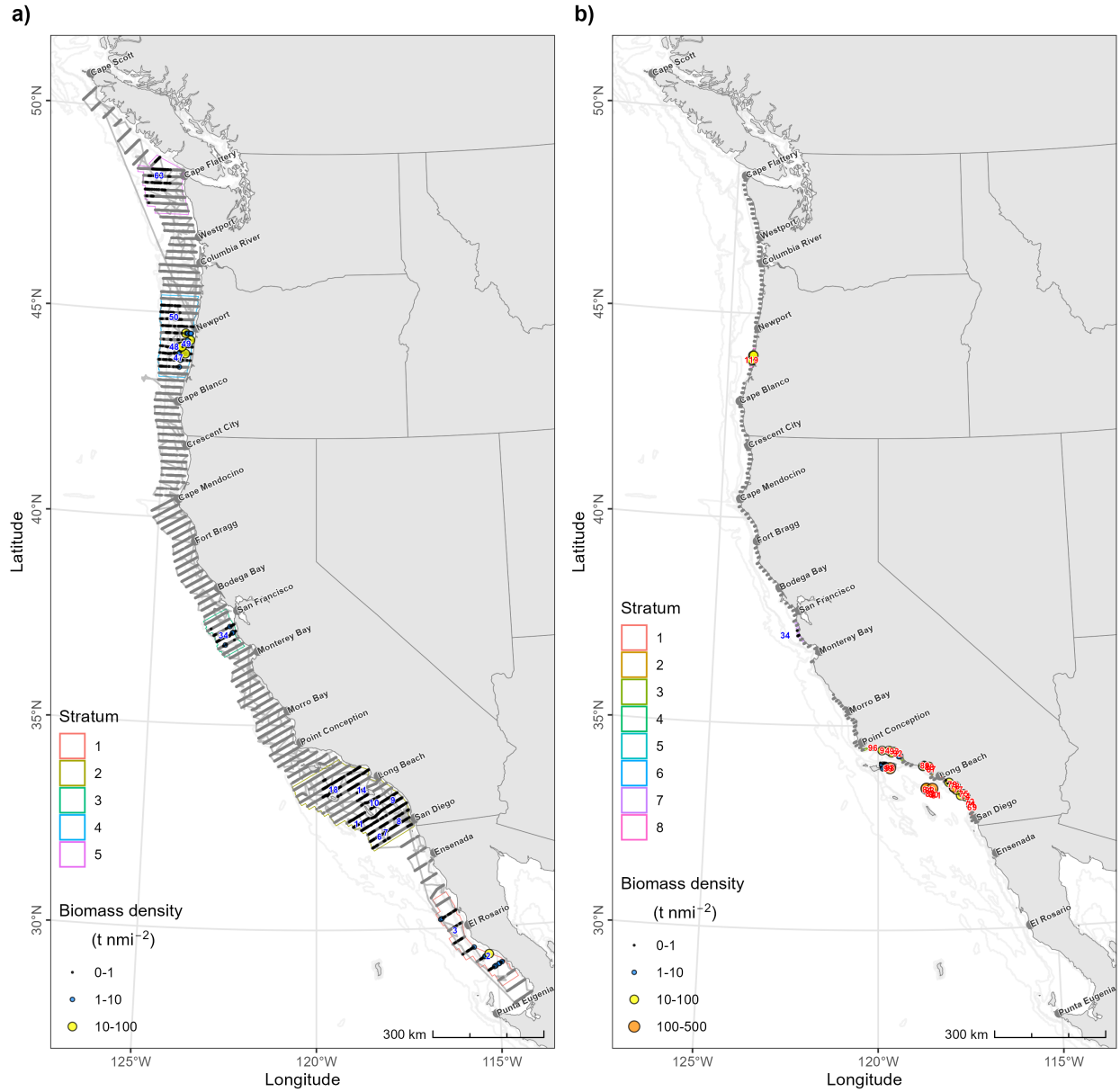
Figure 28: Biomass densities (colored points) of Pacific Mackerel ( Scomber japonicus ), per stratum, in the a) core and b) nearshore survey regions. Overlaid are the locations of trawl clusters (blue numbers) or purse seine samples (red numbers) with at least one Pacific Mackerel in each stratum (colored polygons). Thick gray lines represent acoustic transects.
