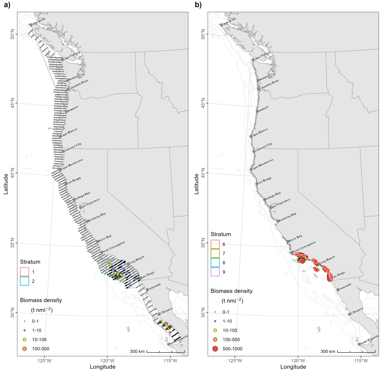
Figure 26: Biomass densities (colored points) of the southern subpopulation of Pacific Sardine ( Sardinops sagax ), per stratum, in the a) core and b) nearshore survey regions. Overlaid are the locations of trawl clusters (blue numbers) or purse seine samples (red numbers) with at least one Pacific Sardine in each stratum (colored polygons). Thick gray lines represent acoustic transects.
