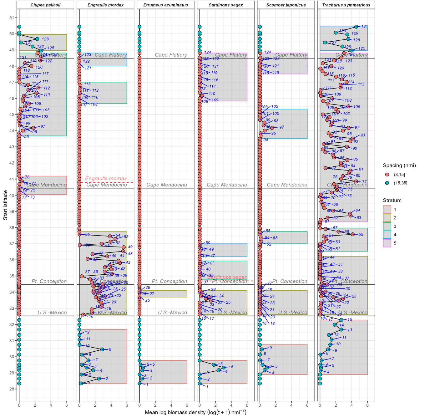
Figure 14: Log-transformed biomass density + 1 ( \log(t + 1) \text{ nmi}^{-2} ) by transect versus latitude (easternmost portion of each transect) and strata (shaded regions; outline indicates stratum number) used to estimate biomass and abundance for each species in the core region surveyed by Lasker . Data labels (blue numbers) correspond to transects with positive biomass ( \log_e(t + 1) > 0 ). Transect spacing (nmi; point color), and subpopulation breaks for Northern Anchovy and Pacific Sardine (red dashed lines and text) are indicated.
