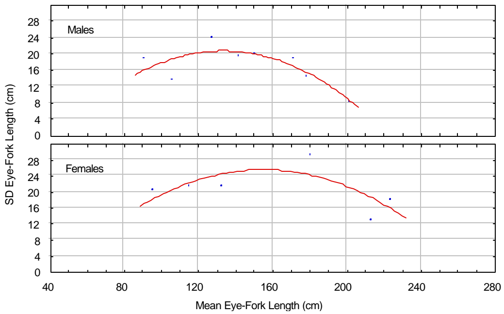
Figure 2. Sample standard deviation (SD) in length-at-age against mean lengths. Solid line indicates trend predicted with quadratic function.
