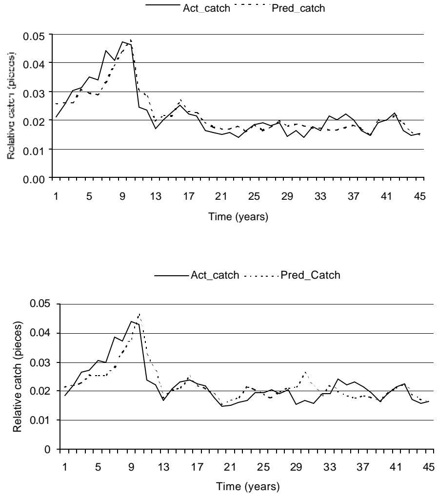
Figure 11. Actual and predicted catch levels based on Japanese and US longline fishing effort only over 1952-1996 (top) and for all fisheries (bottom). Relative catches were obtained by dividing annual catches by the sum of catches over the simulation period. Natural mortality rates for males and females were 0.43 and 0.15 respectively.
