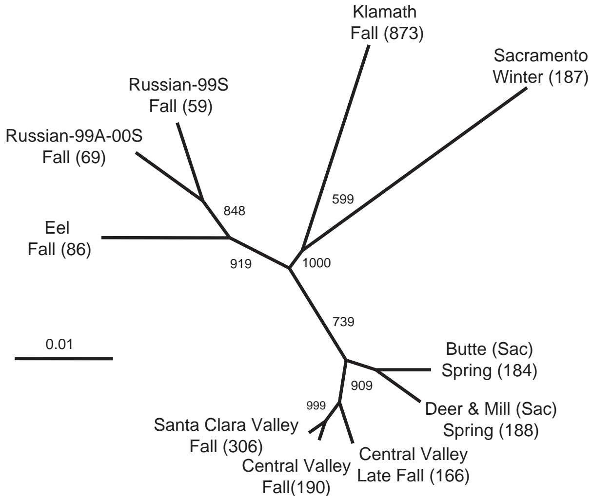
Figure 3.1. Unrooted UPGMA phylogram based on CSE chord distances calculated from data for 7 microsatellite loci, with all Eel River samples pooled. Central Valley data from Banks et al. 2000. Numbers in parentheses indicate sample size. Branch length is scaled to genetic distance (see scale in figure), and numbers at nodes indicate number of bootstrap iterations out of 1000 in which the node occurs. (Redrawn from Figure 9 in Hedgecock (2002)).
