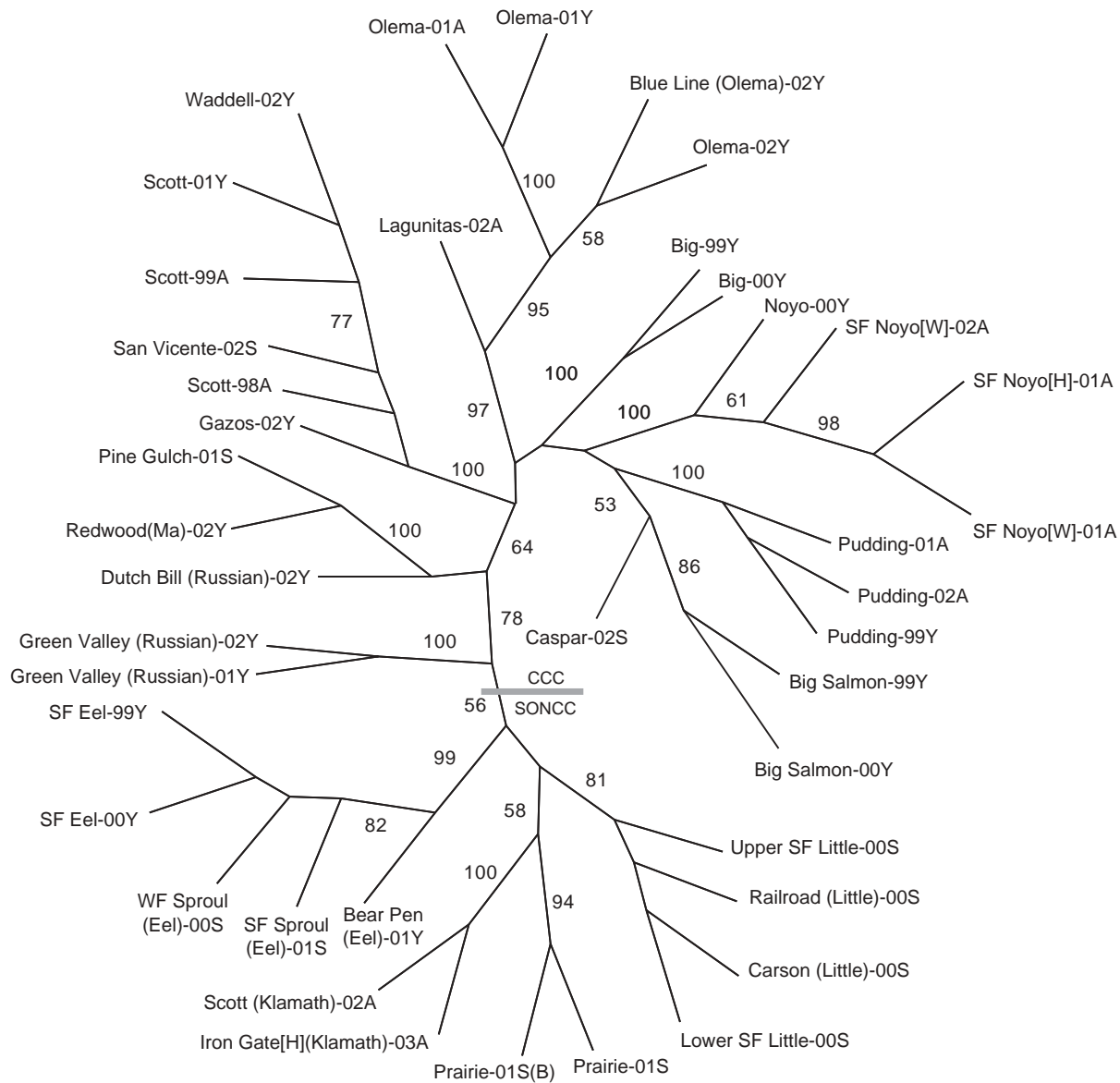
Figure 2.2. Bootstrap consensus tree for coho salmon in California. Consensus tree is based on trees constructed with a neighbor-joining algorithm (Saitou and Nei, 1987) using Cavalli-Sforza and Edwards (1967) chord distances calculated for 5000 data sets generated by bootstrap resampling from data for 18 microsatellite loci. Numbers on internal branches indicate the proportion (>50%) of trees in which the indicated node appeared. Samples are identified by stream, brood year, life stage (“A” indicates adult; “S” indicates smolt or outmigrating juvenile; “Y” indicates young-of-year juvenile), and where appropriate, as being collected from hatchery “[H]” or wild “[W]” populations. Parenthetical information indicates tributary basin (where relevant) or county.
