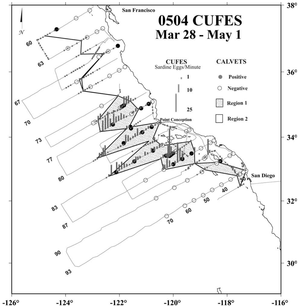
Figure 1. Sardine eggs from CalVET, a.k.a. Pairovet; (solid circle denotes positive catch and open circle denotes zero catch) and from CUFES (stick denotes positive collection) in March-April 2005 survey. The numbers on line 93 are CalCOFI station numbers. Region 1 is stippled area.
