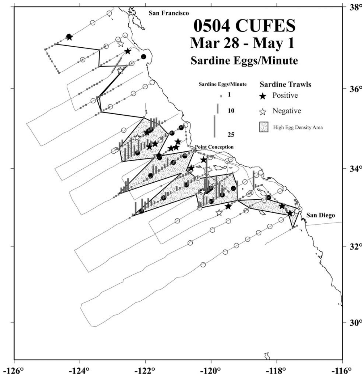
Figure 4. March-April 2005 trawl start locations. Solid stars are trawls that contained at least one sardine. Background is CUFES track lines and sardine egg abundance, pair-ovet tows (circles: solid are positive for sardine eggs or larvae; open are negative). The high egg density area is Region 1.
