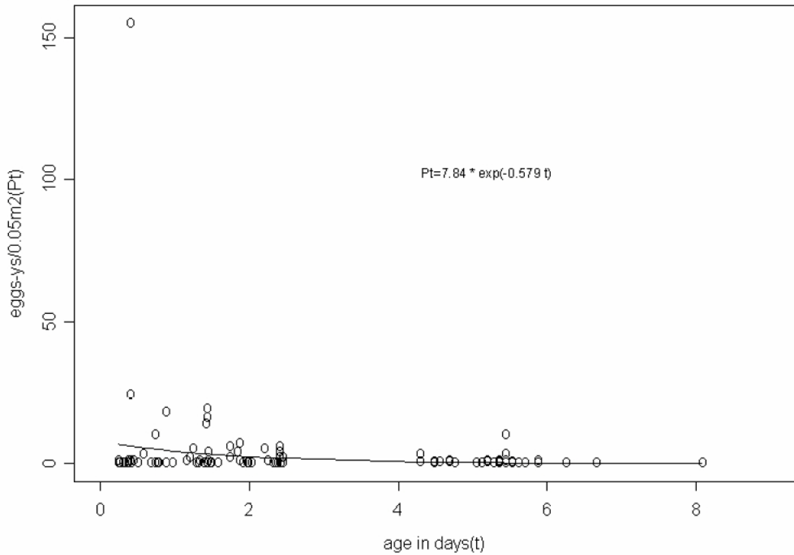
Figure 6. Embryonic mortality curve of Pacific sardine. Staged egg data were from CalVET and yolk-sac larval data were from CalVET and Bongo in 2005. The number, 7.84, is the estimate of daily egg production before correction for bias.
