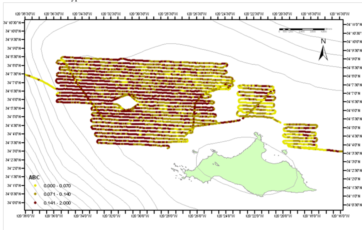
Figure 1.25. Northwest, North and Northeast San Miguel Island area backscatter coefficients ( s_u ; m^2/m^2 ) attributed to seabed type.
