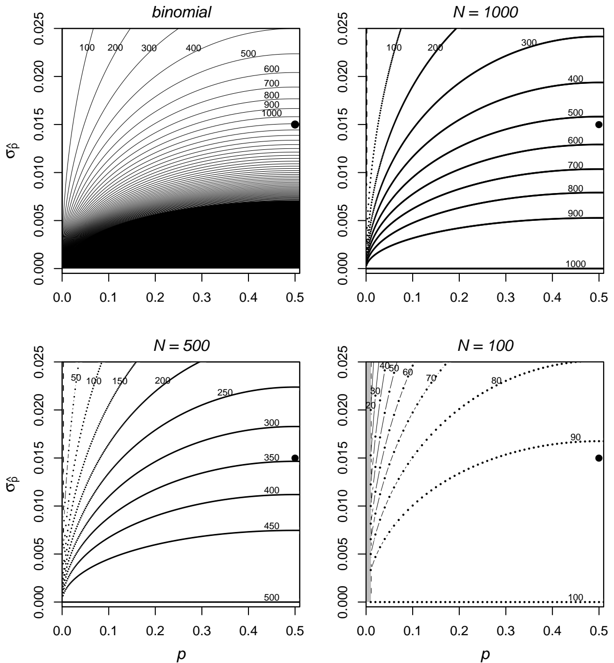
Figure 3. Sample size (contours) required to yield a specified \sigma_{\hat{p}} , given the stock proportion p . Top-left panel presents results for binomial sampling; remaining panels give hypergeometric results for total landings of 1000, 500, and 100 fish, respectively. In the hypergeometric panels, p less than the minimum non-zero value possible ( \frac{1}{N} ) are block-shaded in grey, and for contoured values of n the possible (n, p) combinations appear as black dots connected by line segments (for larger N, n appearing as a nearly continuous line over the range displayed, 0 \leq p \leq 0.5 ). Large dot marks criterion described in the text ( \sigma_{\hat{p}} = 0.015 for p = 0.5 ).
