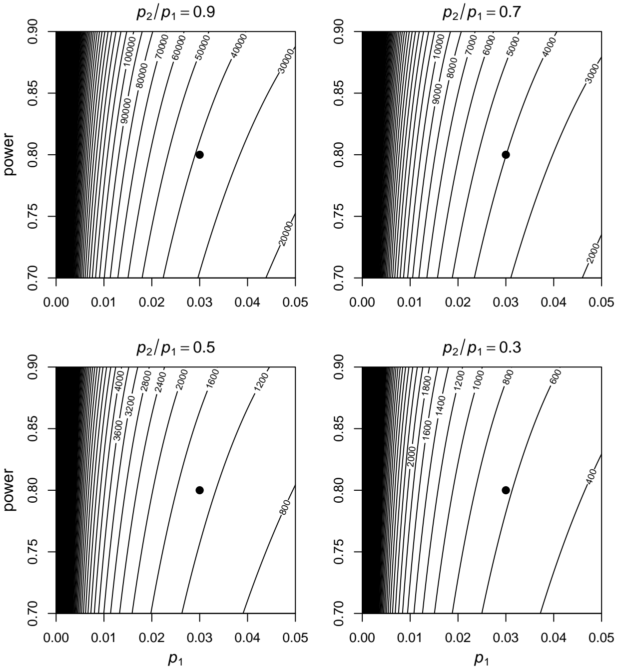
Figure 4. Sample size (contours) required to yield a specified power (with \alpha = 0.05 ) to detect a difference in two stock proportions, given the larger proportion p_1 , and the ratio of the two proportions \frac{p_2}{p_1} (different panels). Sample size indicated is required for each of the two independent binomial samples. Large dot marks criterion described in the text (power = 0.8 for p_1 = 0.03 ).
