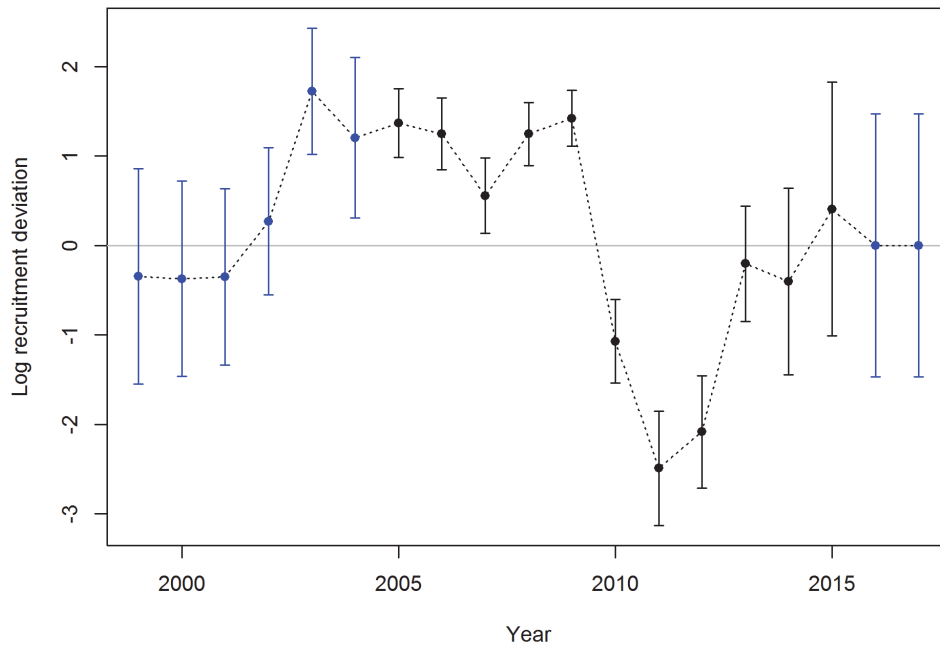
Figure 29. Recruitment deviations and standard errors ( \sigma_R = 0.75 ) for model ALT. Year labels represent year of SSB producing the subsequent year class.
