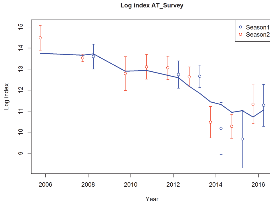
Figure 27. Fit to the AT survey abundance index in arithmetic (upper panel) and log (lower panel) scales for model ALT. Q=1.1 (estimated).
