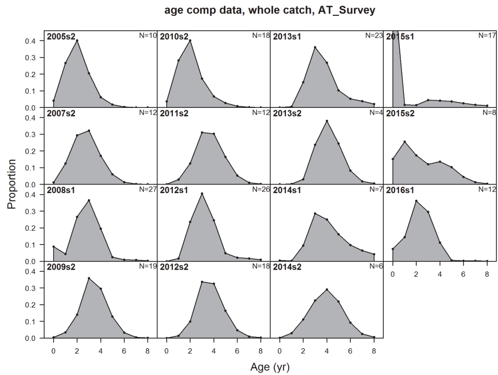
Figure 12. Length- (upper panel) and age-composition (lower panel) time series for the AT survey. N represents input sample sizes.
